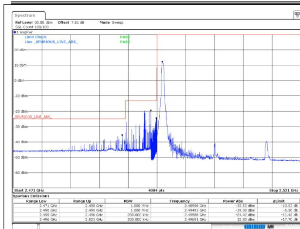
n41 SCS=30kHz DFT_16QAM BW=20MHz LowChannel=501204 RB=1@0
