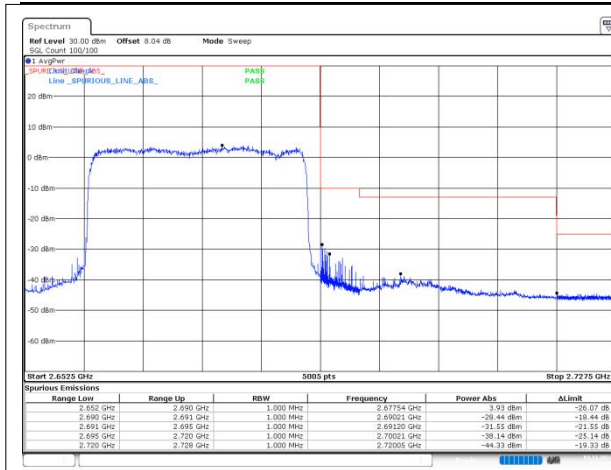
n41 SCS=30kHz DFT_BPSK BW=30MHz HighChannel=534996 RB=75@0
