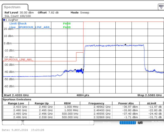
n41 SCS=30kHz DFT_64QAM BW=50MHz LowChannel=504204 RB=128@0
