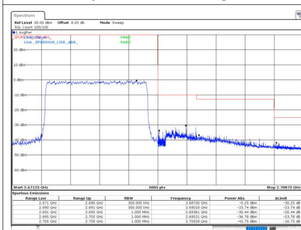
n41 SCS=30kHz DFT_16QAM BW=15MHz HighChannel=536496 RB=36@0
