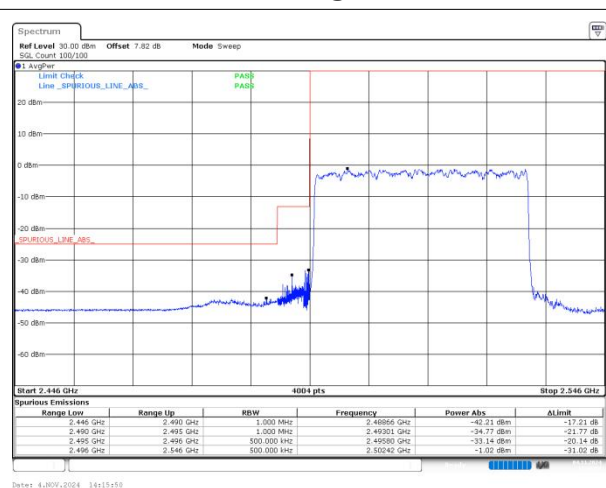
n41 SCS=30kHz DFT_BPSK BW=40MHz LowChannel=503202 RB=100@0
