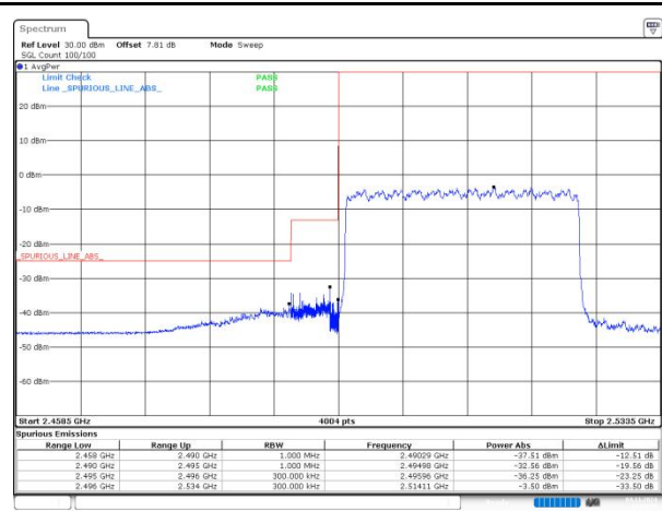
n41 SCS=30kHz DFT_64QAM BW=30MHz LowChannel=502200 RB=75@0
