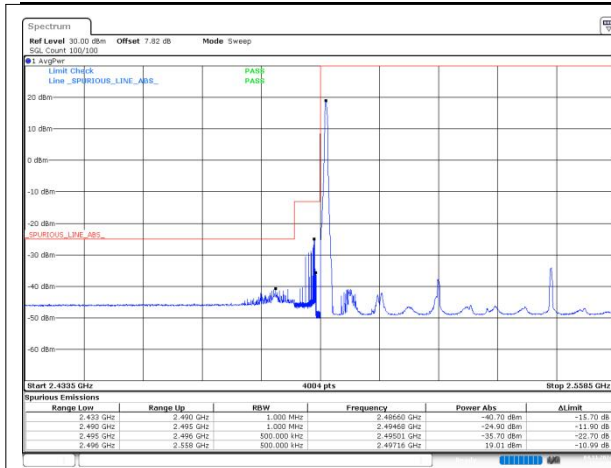
n41 SCS=30kHz DFT_16QAM BW=50MHz LowChannel=504204 RB=1@0
