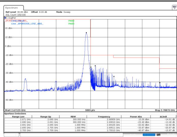
n41 SCS=30kHz DFT_16QAM BW=15MHz HighChannel=536496 RB=1@37
