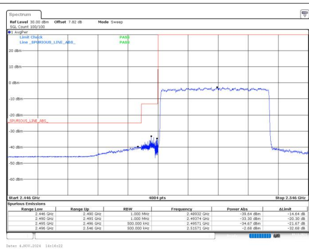
n41 SCS=30kHz DFT_16QAM BW=40MHz LowChannel=503202 RB=100@0
