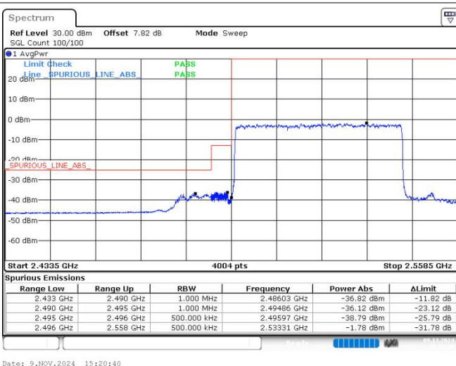
n41 SCS=30kHz DFT_256QAM BW=50MHz LowChannel=504204 RB=128@0
