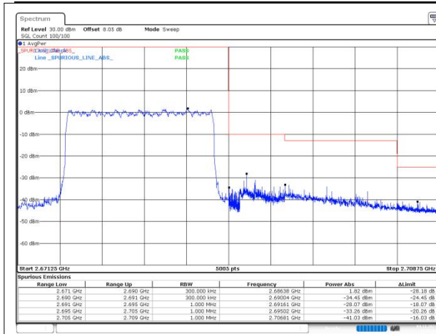
n41 SCS=30kHz DFT_QPSK BW=15MHz HighChannel=536496 RB=36@0
