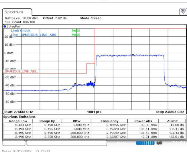
n41 SCS=30kHz DFT_BPSK BW=50MHz LowChannel=504204 RB=128@0
