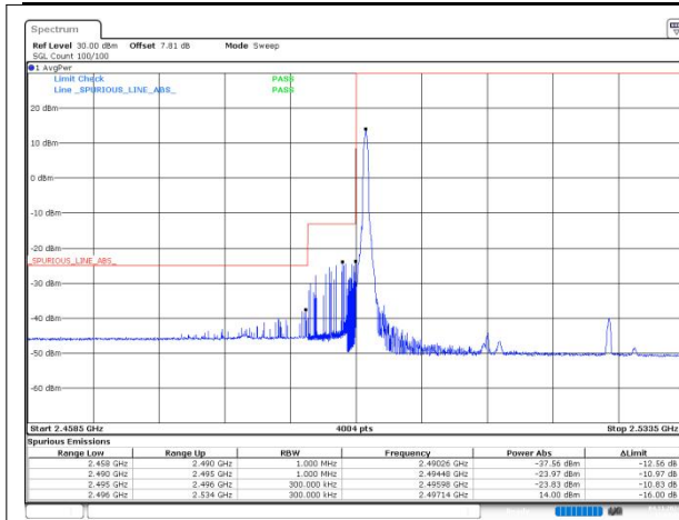
n41 SCS=30kHz DFT_64QAM BW=30MHz LowChannel=502200 RB=1@0
