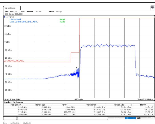
n41 SCS=30kHz DFT_64QAM BW=40MHz LowChannel=503202 RB=100@0
