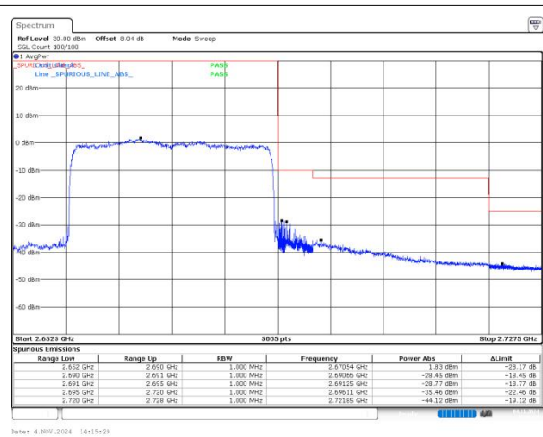
n41 SCS=30kHz CP_QPSK BW=30MHz HighChannel=534996 RB=78@0
