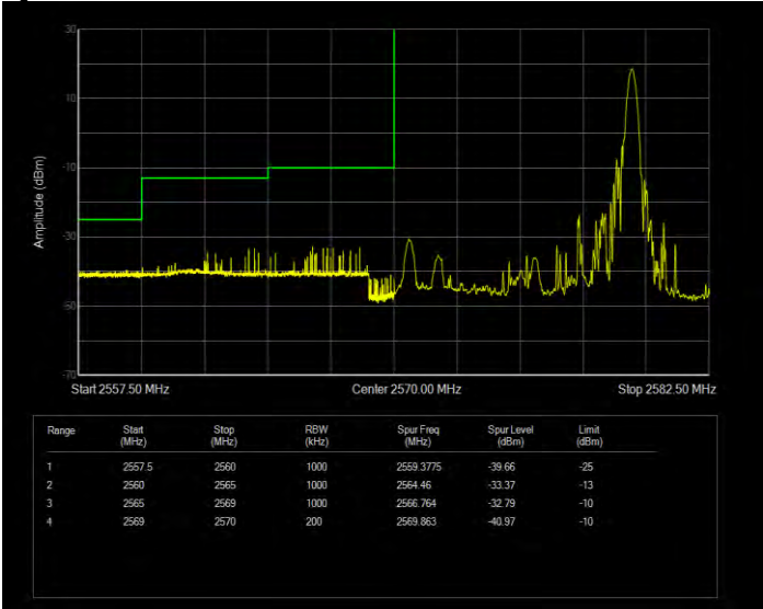
Band38 QPSK BW=10MHz Channel=37800 RB Size=50 Position=#0 Extended
