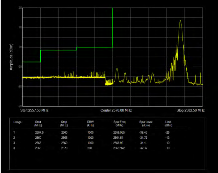
Band38 16QAM BW=10MHz Channel=37800 RB Size=50 Position=#0 Extended
