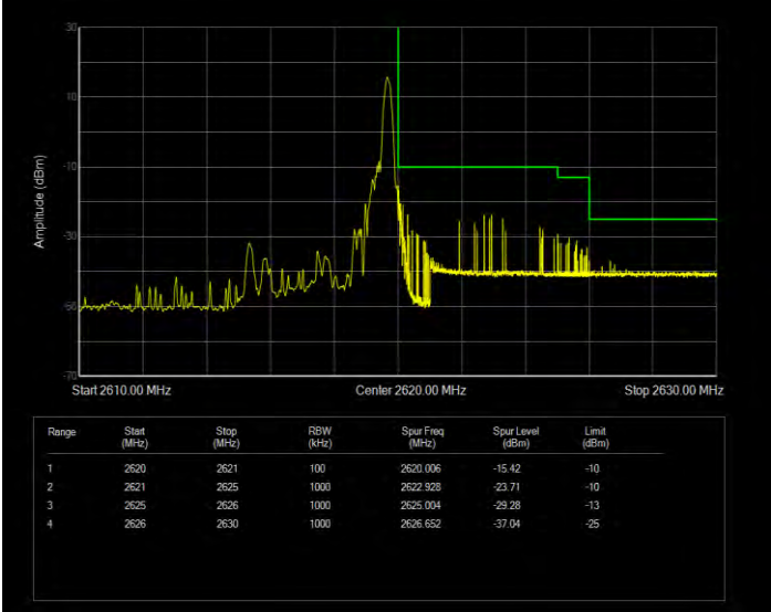
Band38 16QAM BW=5MHz Channel=38225 RB Size=25 Position=#0 Extended
