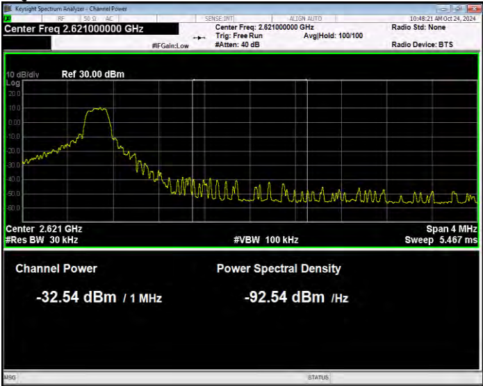
Band38 16QAM BW=5MHz Channel=38225 RB Size=1 Position=#Max Extended
