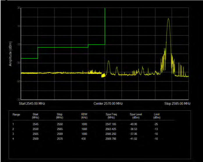
Band38 QPSK BW=20MHz Channel=37850 RB Size=100 Position=#0 Extended
