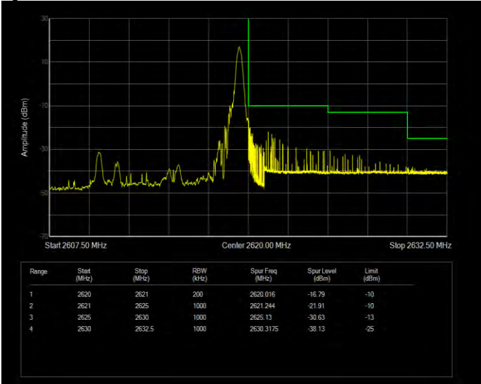
Band38 QPSK BW=10MHz Channel=38200 RB Size=50 Position=#0 Extended
