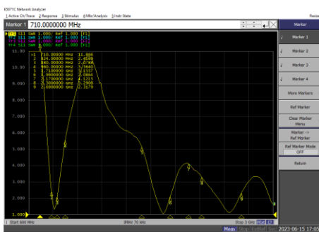
P10 ANT1 VSWR/Return Loss
