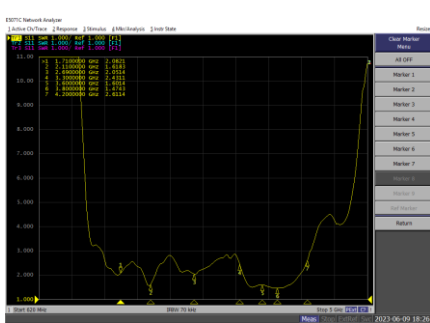
P10 ANT3 VSWR/Return Loss
