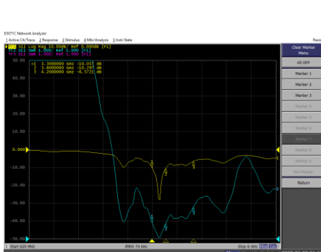
P10 ANT5 VSWR/Return Loss
