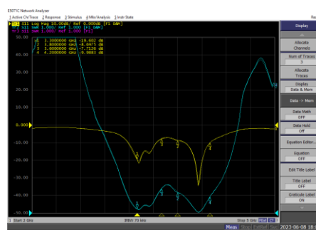
P10 ANT4 VSWR/Return Loss
