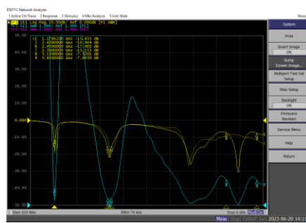
P10 WIFI 2 VSWR/Return Loss
