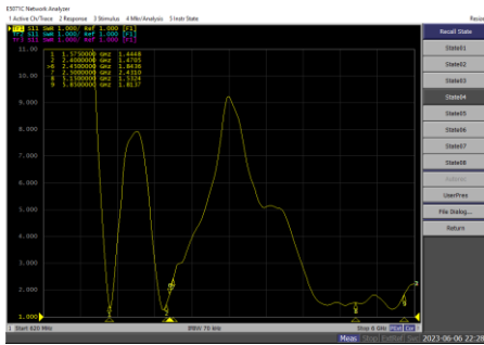
P10 WIFI 1 VSWR/Return Loss
