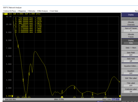
P10 ANT6 VSWR/Return Loss
