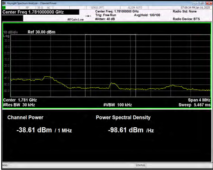
Band66 16QAM BW=3MHz Channel=132657 RB Size=1 Position=#0 Extended
