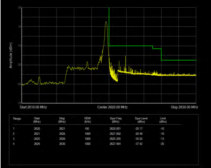
Band38 QPSK BW=5MHz Channel=38225 RB Size=25 Position=#0 Extended
