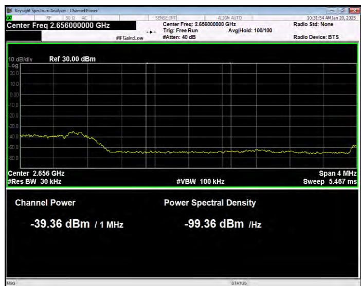
Band41(2555-2655) QPSK BW=5MHz Channel=41215 RB Size=1 Position=#0 Normal
