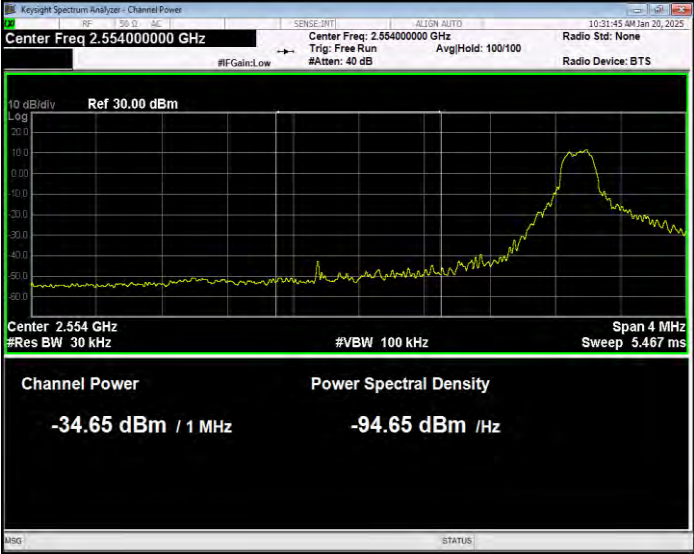
Band41(2555-2655) 16QAM BW=5MHz Channel=40265 RB Size=1 Position=#0 Normal
