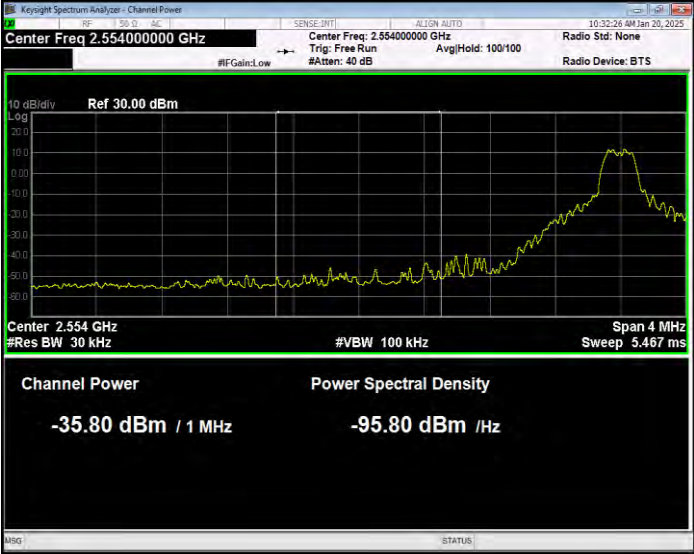
Band41(2555-2655) 16QAM BW=10MHz Channel=40290 RB Size=1 Position=#0 Normal
