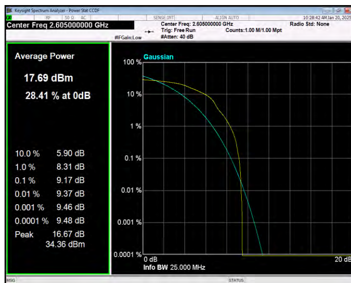
Band41(2555-2655) QPSK BW=10MHz Channel=40740 RB Size=1 Position=#0
