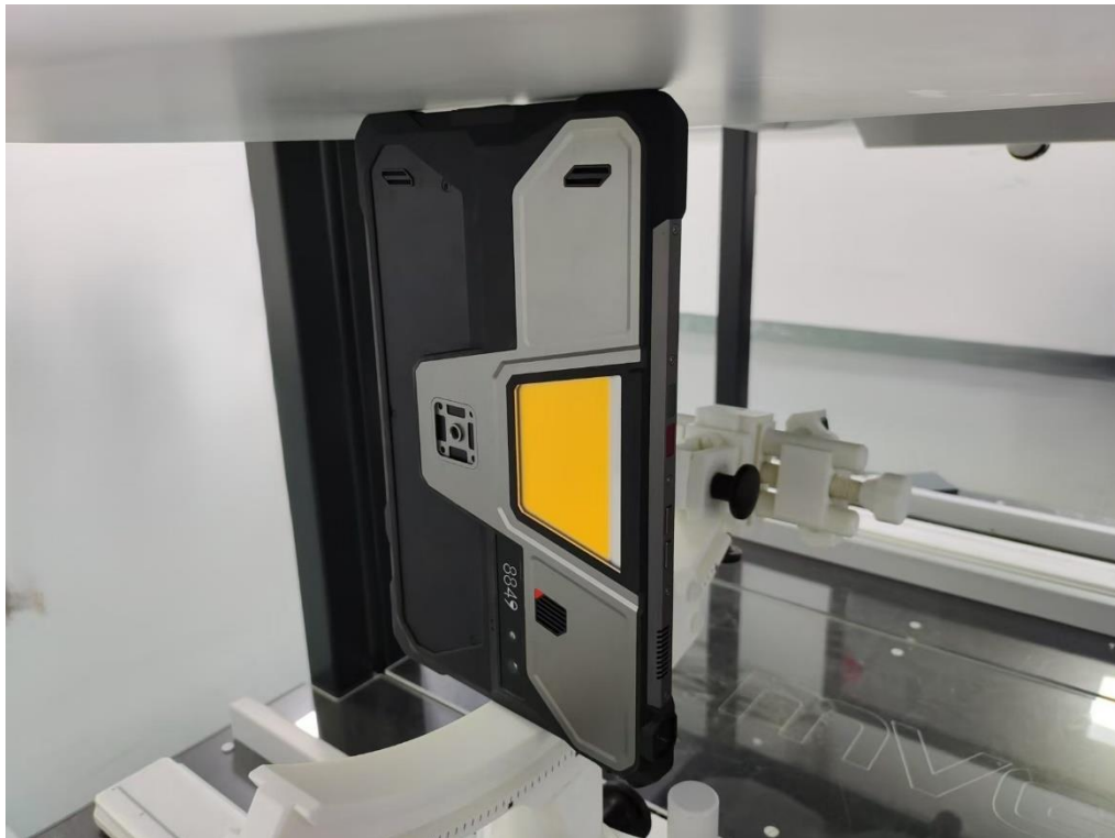
Body Bottom side (separation distance 0mm)
