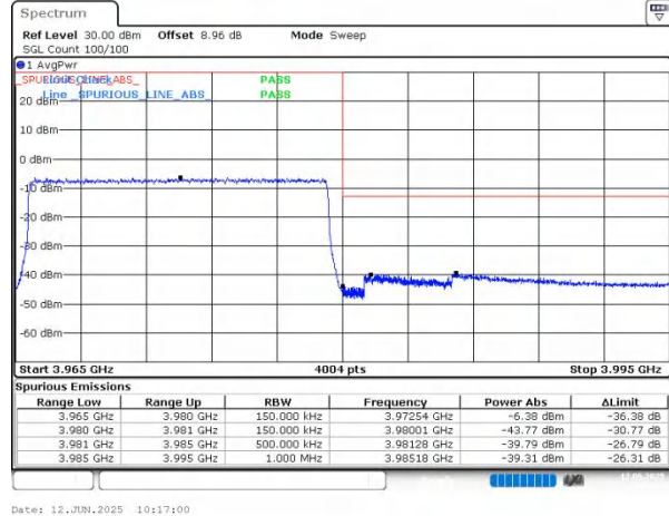
n77(3700-3980) SCS=30kHz CP_QPSK BW=15MHz HighChannel=664832 RB=38@0
