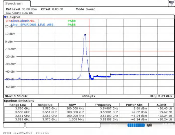
n78(3450-3550) SCS=30kHz DFT_64QAM BW=20MHz HighChannel=636000 RB=1@50
