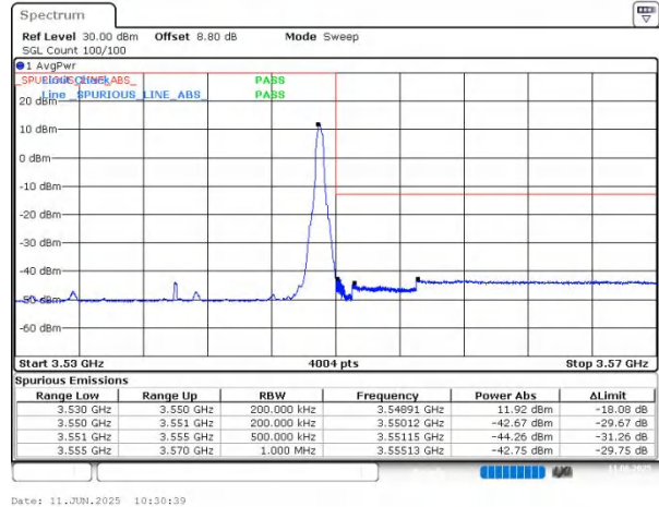
n78(3450-3550) SCS=30kHz DFT_QPSK BW=20MHz HighChannel=636000 RB=1@50
