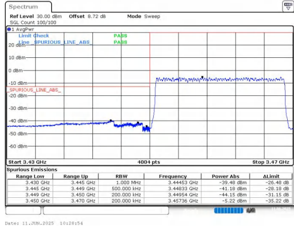
n78(3450-3550) SCS=30kHz DFT_64QAM BW=20MHz LowChannel=630668 RB=50@0
