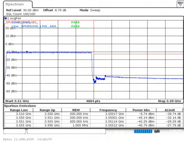
n78(3450-3550) SCS=30kHz CP_QPSK BW=40MHz HighChannel=635332 RB=106@0
