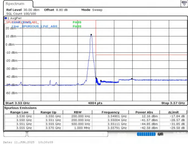
n78(3450-3550) SCS=30kHz DFT_BPSK BW=20MHz HighChannel=636000 RB=1@50
