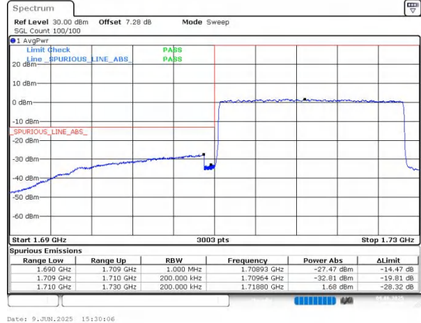
n66 SCS=15kHz DFT_64QAM BW=20MHz LowChannel=344000 RB=100@0
