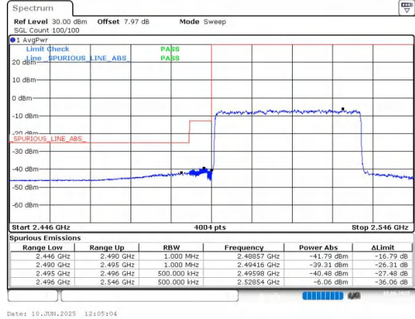
n41 SCS=30kHz DFT_256QAM BW=40MHz LowChannel=503202 RB=100@0
