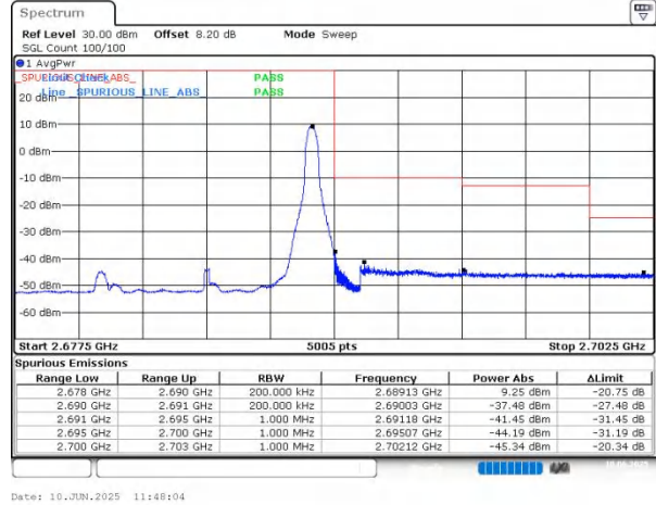
n41 SCS=30kHz DFT_256QAM BW=10MHz HighChannel=537000 RB=1@23
