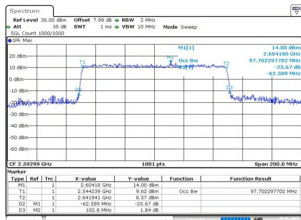
n41 SCS=30kHz DFT_BPSK BW=100MHz Channel=518598 RB=270@0
