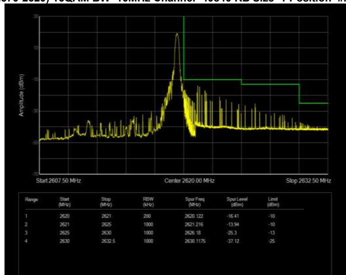
Band41(2570-2620) 16QAM BW=10MHz Channel=40840 RB Size=50 Position=#0 Normal
