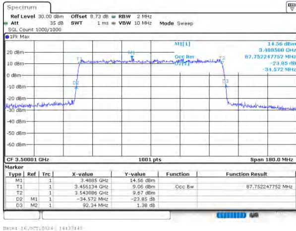
n78(3450-3550) SCS=30kHz CP_16QAM BW=90MHz Channel=633334 RB=245@0
