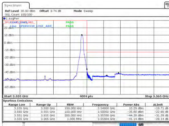
n78(3450-3550) SCS=30kHz DFT_16QAM BW=15MHz HighChannel=636166 RB=1@37
