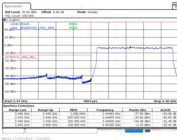
n78(3450-3550) SCS=30kHz DFT_BPSK BW=10MHz LowChannel=630334 RB=24@0
