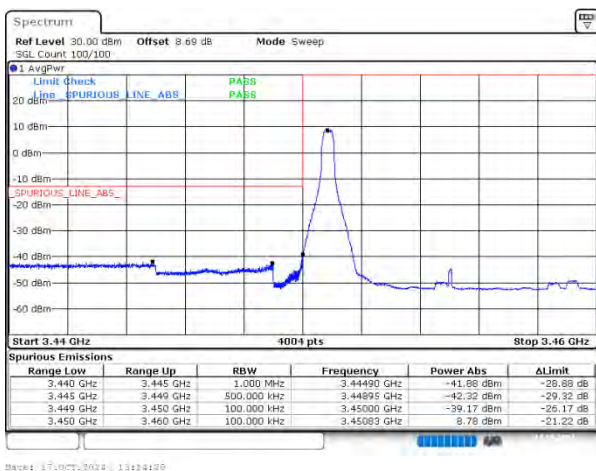
n78(3450-3550) SCS=30kHz DFT_16QAM BW=10MHz LowChannel=630334 RB=1@0
