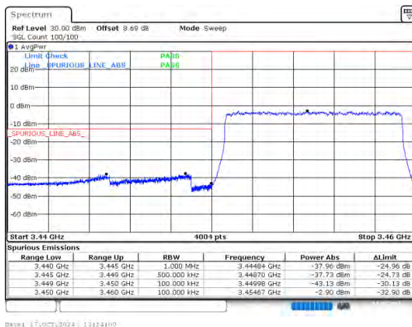
n78(3450-3550) SCS=30kHz DFT_QPSK BW=10MHz LowChannel=630334 RB=24@0
