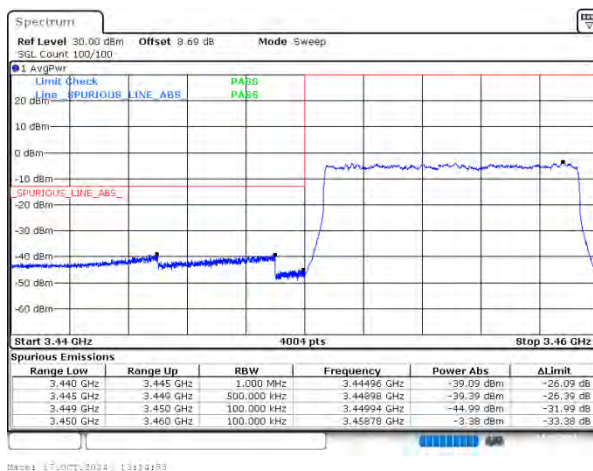
n78(3450-3550) SCS=30kHz DFT_16QAM BW=10MHz LowChannel=630334 RB=24@0
