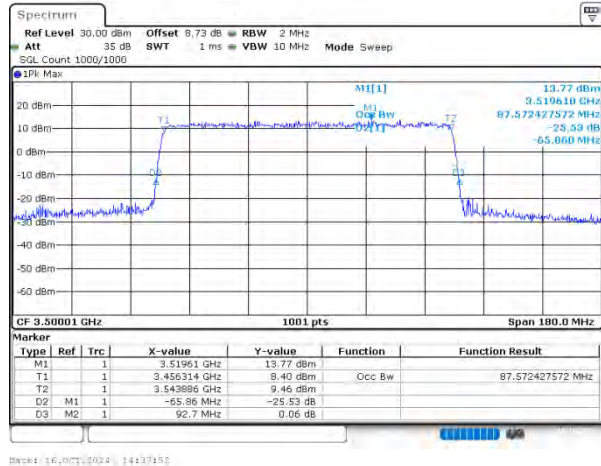
n78(3450-3550) SCS=30kHz CP_64QAM BW=90MHz Channel=633334 RB=245@0
