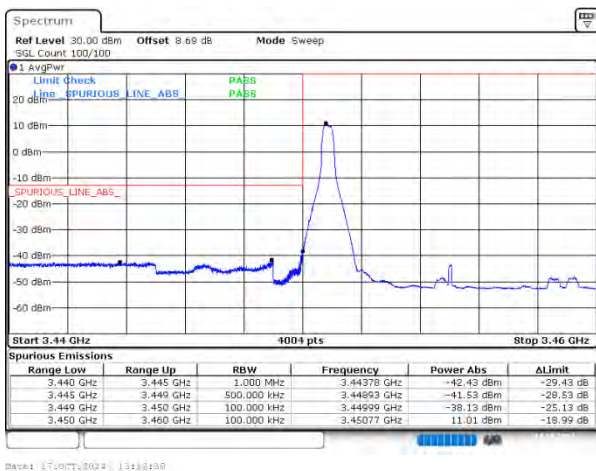
n78(3450-3550) SCS=30kHz DFT_BPSK BW=10MHz LowChannel=630334 RB=1@0
