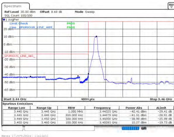
n78(3450-3550) SCS=30kHz DFT_QPSK BW=10MHz LowChannel=630334 RB=1@0
