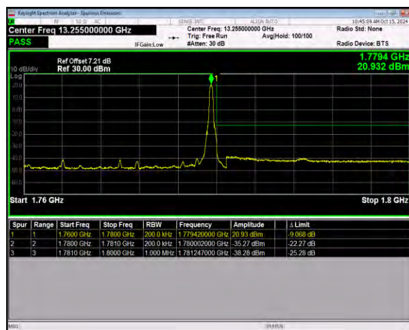
n66 SCS=15kHz DFT_QPSK BW=20MHz HighChannel=354000 RB=1@105
