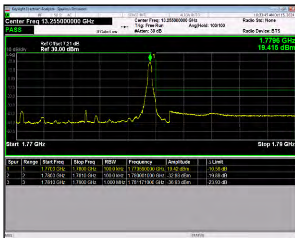
n66 SCS=15kHz DFT_BPSK BW=10MHz HighChannel=355000
