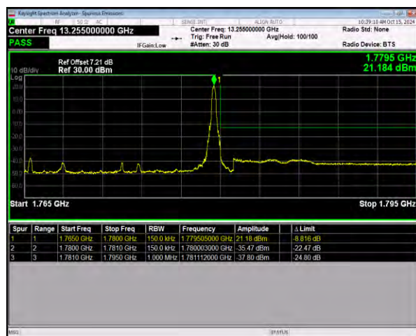
n66 SCS=15kHz DFT_BPSK BW=15MHz HighChannel=354500 RB=1@78
