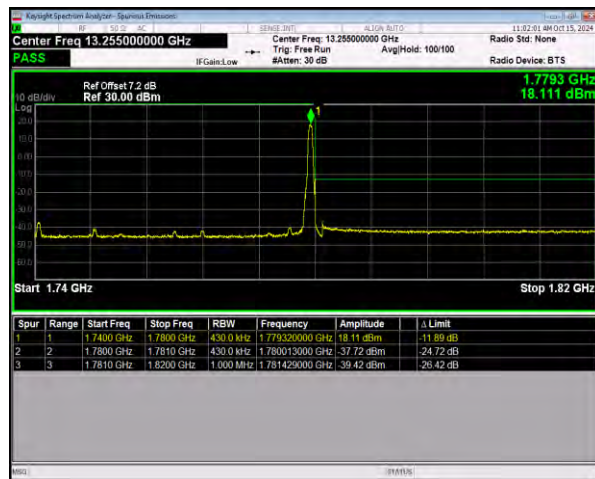
n66 SCS=15kHz DFT_256QAM BW=40MHz HighChannel=352000 RB=1@215
