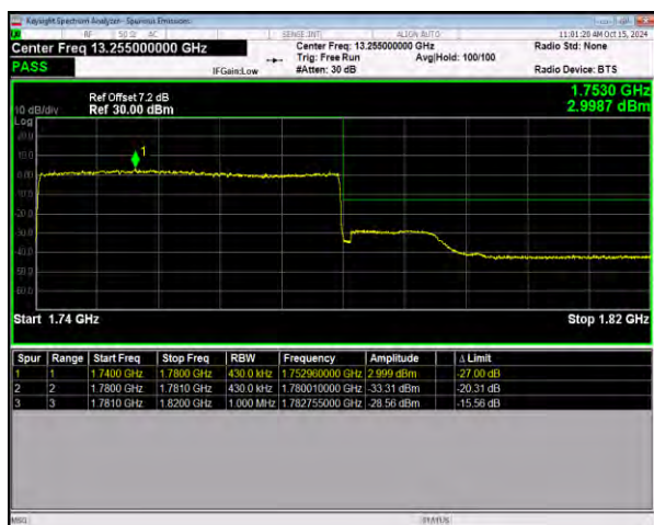
n66 SCS=15kHz DFT_16QAM BW=40MHz HighChannel=352000 RB=216@0
