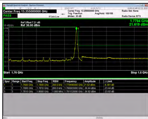
n66 SCS=15kHz DFT_BPSK BW=20MHz HighChannel=354000
