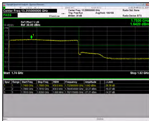
n66 SCS=15kHz CP_QPSK BW=40MHz HighChannel=352000 RB=216@0
