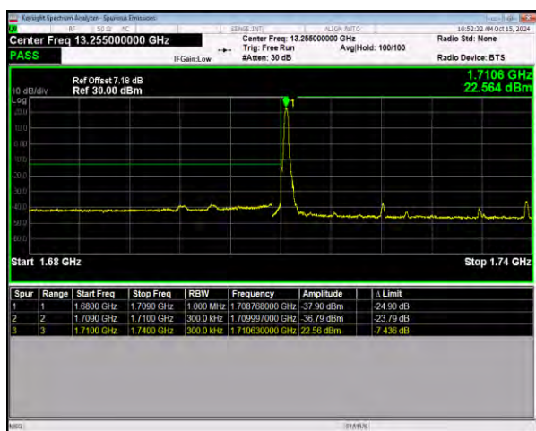
n66 SCS=15kHz DFT_BPSK BW=30MHz LowChannel=345000 RB=1@0
