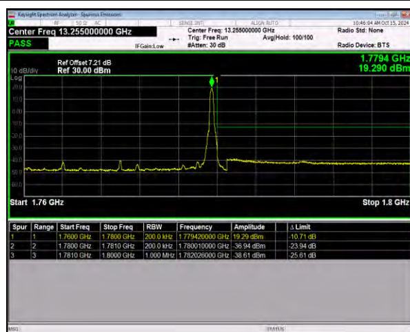
n66 SCS=15kHz DFT_64QAM BW=20MHz HighChannel=354000 RB=1@105
