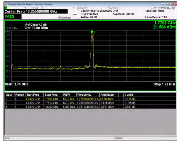
n66 SCS=15kHz DFT_QPSK BW=40MHz HighChannel=352000 RB=1@215
