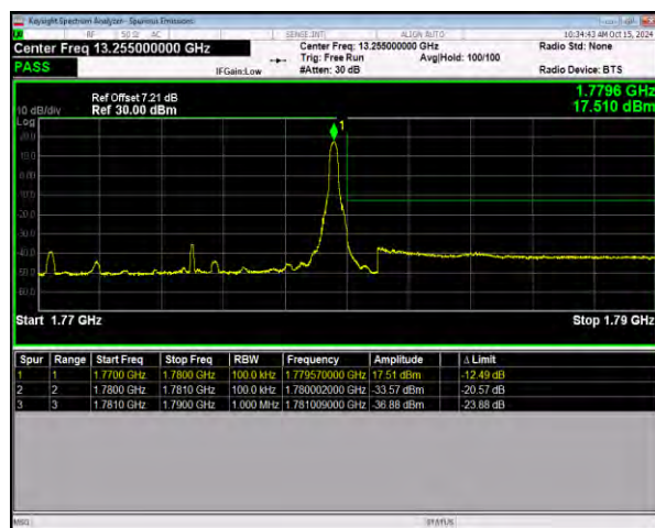
n66 SCS=15kHz DFT_16QAM BW=10MHz HighChannel=355000 RB=1@51
