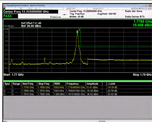
n66 SCS=15kHz DFT_256QAM BW=10MHz HighChannel=355000 RB=1@51
