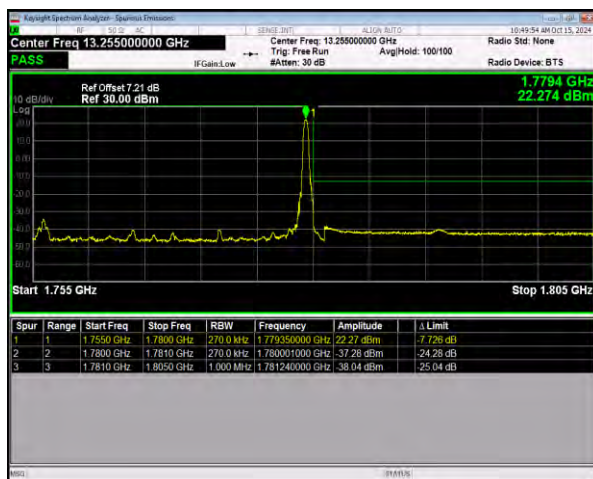
n66 SCS=15kHz DFT_BPSK BW=25MHz HighChannel=353500
