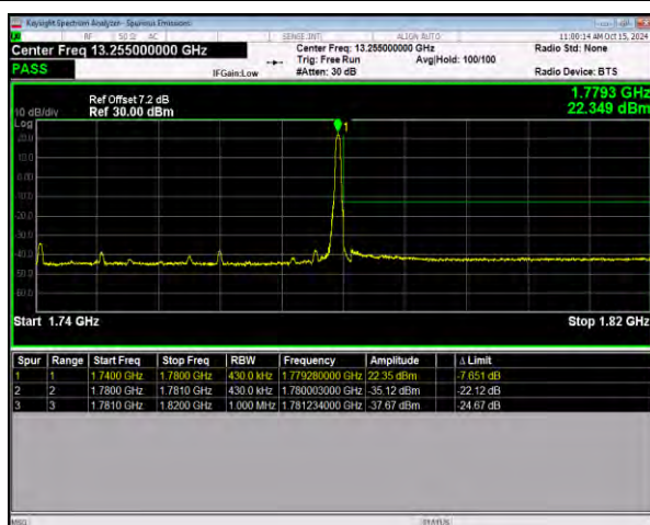
n66 SCS=15kHz DFT_BPSK BW=40MHz HighChannel=352000
