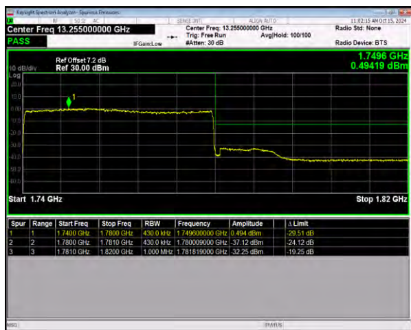
n66 SCS=15kHz DFT_256QAM BW=40MHz HighChannel=352000 RB=216@0
