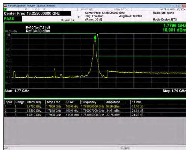
n66 SCS=15kHz DFT_64QAM BW=10MHz HighChannel=355000 RB=1@51
