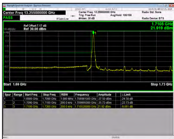
n66 SCS=15kHz DFT_BPSK BW=20MHz LowChannel=344000 RB=1@0
