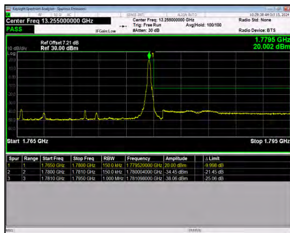
n66 SCS=15kHz DFT_QPSK BW=15MHz HighChannel=354500 RB=1@78
