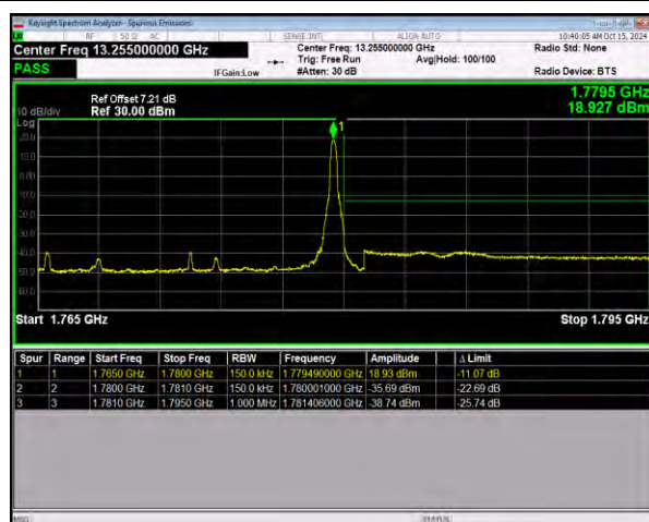
n66 SCS=15kHz DFT_16QAM BW=15MHz HighChannel=354500 RB=1@78
