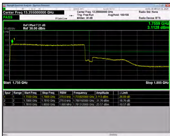
n66 SCS=15kHz DFT_64QAM BW=25MHz HighChannel=353500 RB=128@0
