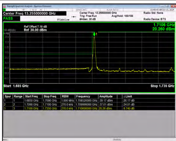
n66 SCS=15kHz DFT_64QAM BW=25MHz LowChannel=344500 RB=1@0
