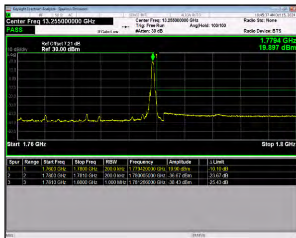
n66 SCS=15kHz DFT_16QAM BW=20MHz HighChannel=354000 RB=1@105
