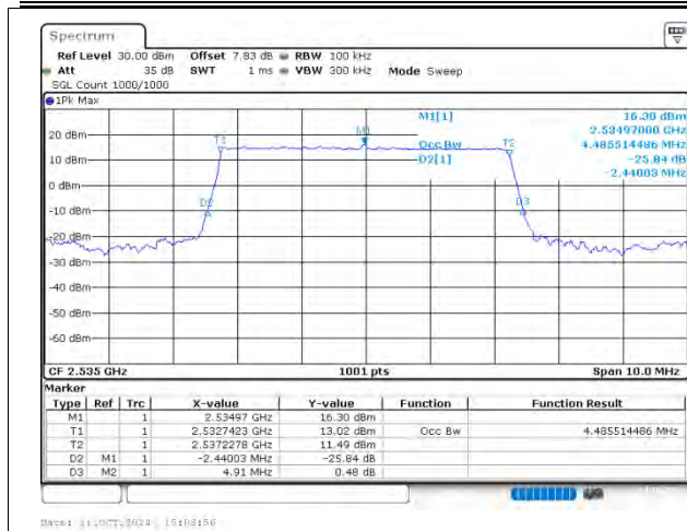
n7 SCS=15kHz DFT_BPSK BW=5MHz Channel=507000 RB=25@0
