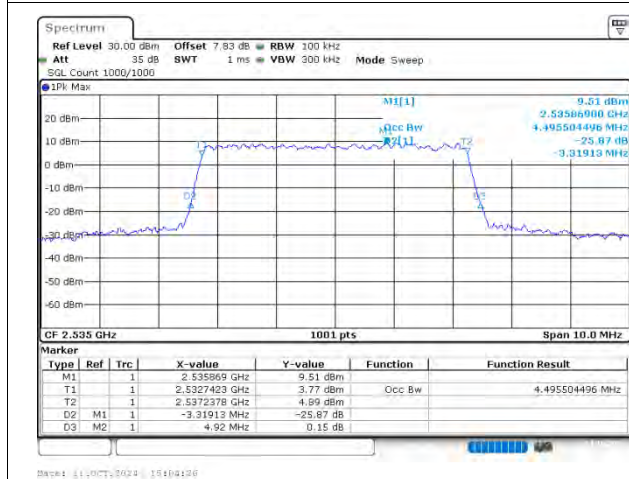
n7 SCS=15kHz CP_256QAM BW=5MHz Channel=507000 RB=25@0
