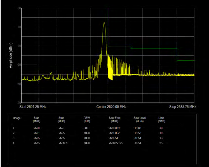
Band38 QPSK BW=15MHz Channel=38175 RB Size=75 Position=#0 Extended
