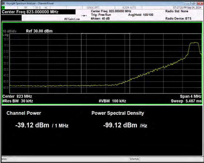
Band26(824-849) QPSK BW=15MHz Channel=26865 RB Size=1 Position=#0 Normal
