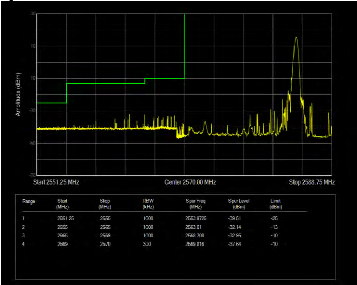
Band38 QPSK BW=15MHz Channel=37825 RB Size=75 Position=#0 Extended
