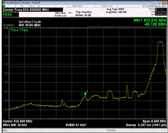
Band26(824-849) QPSK BW=3MHz Channel=26805 RB Size=15 Position=#0 Extended
