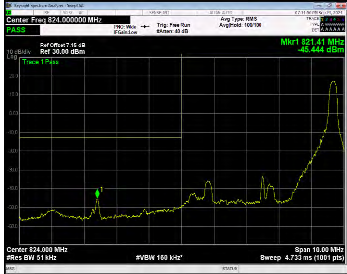
Band26(824-849) QPSK BW=5MHz Channel=26815 RB Size=25 Position=#0 Extended
