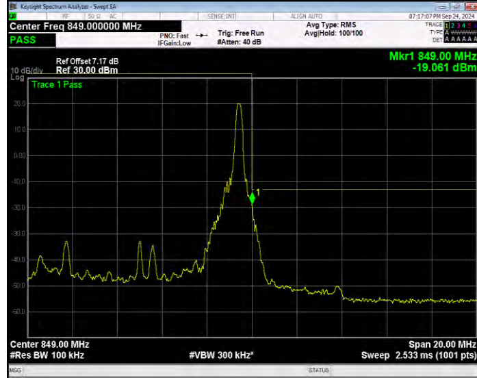
Band26(824-849) 16QAM BW=10MHz Channel=26990 RB Size=50 Position=#0 Extended
