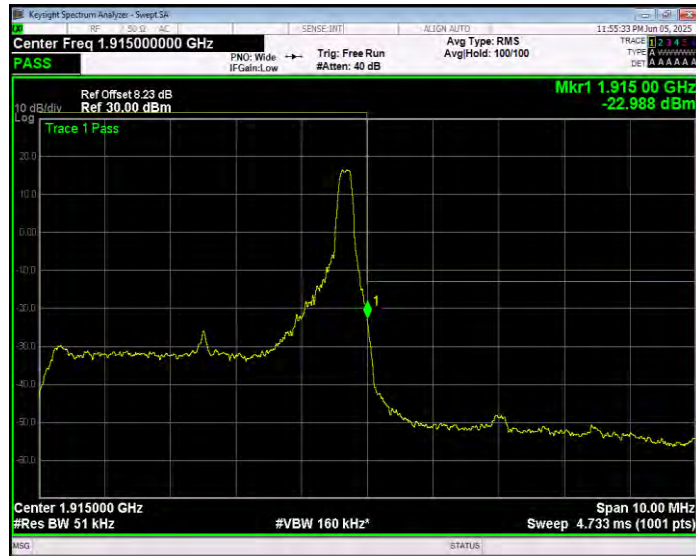
Band25 16QAM BW=5MHz Channel=26665 RB Size=25 Position=#0 Extended
