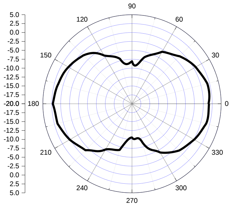
Radiation Pattern (E -Plane): \phi @2.45GHz
