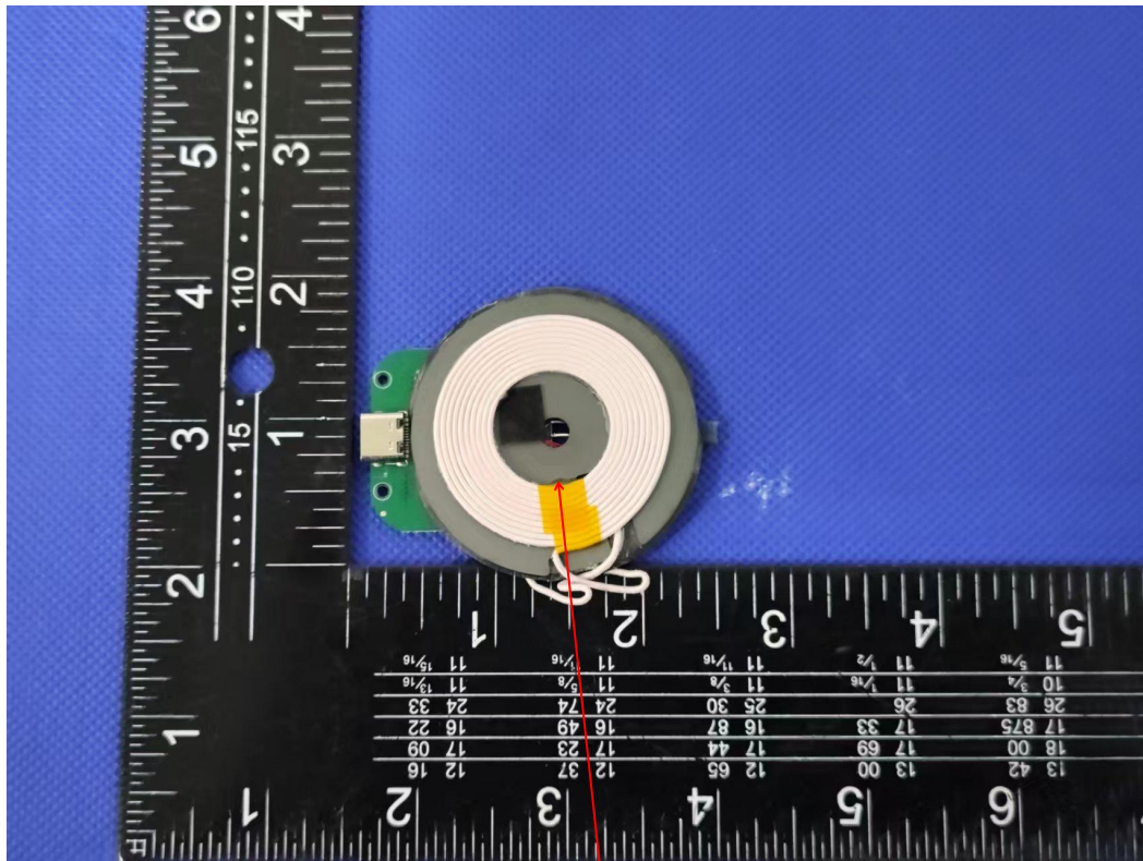
Loop Antenna
