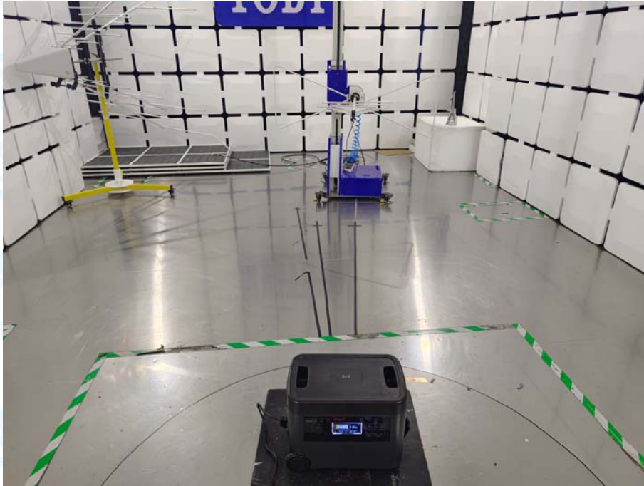
Photo of Setup for Radiated Emission (9KHz-30MHz)
