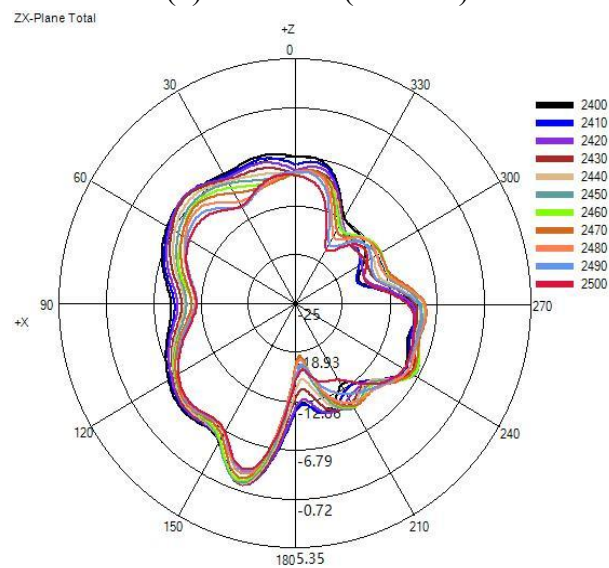
(1) X-Z Plane(unit:dBi):
