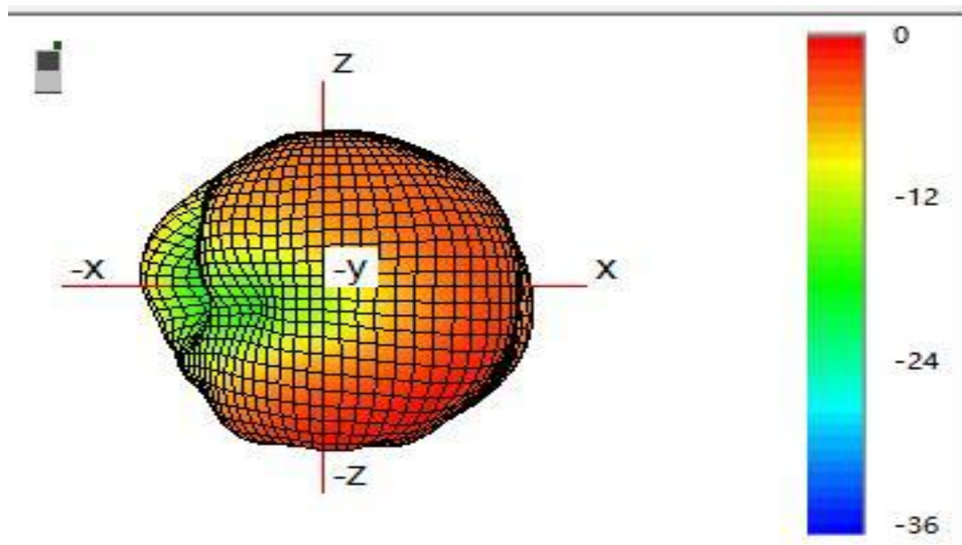
(8) Typical Free Space 3D Radiation Pattern at 2.4GHz(unit:dBi):
