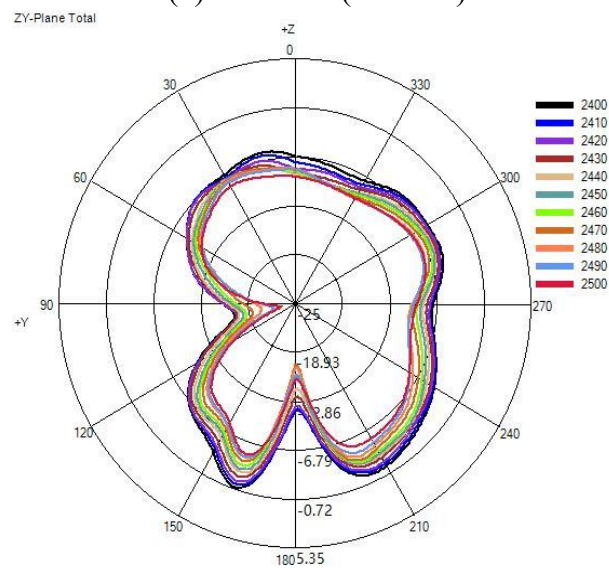
(2) Y-Z Plane(unit:dBi):
