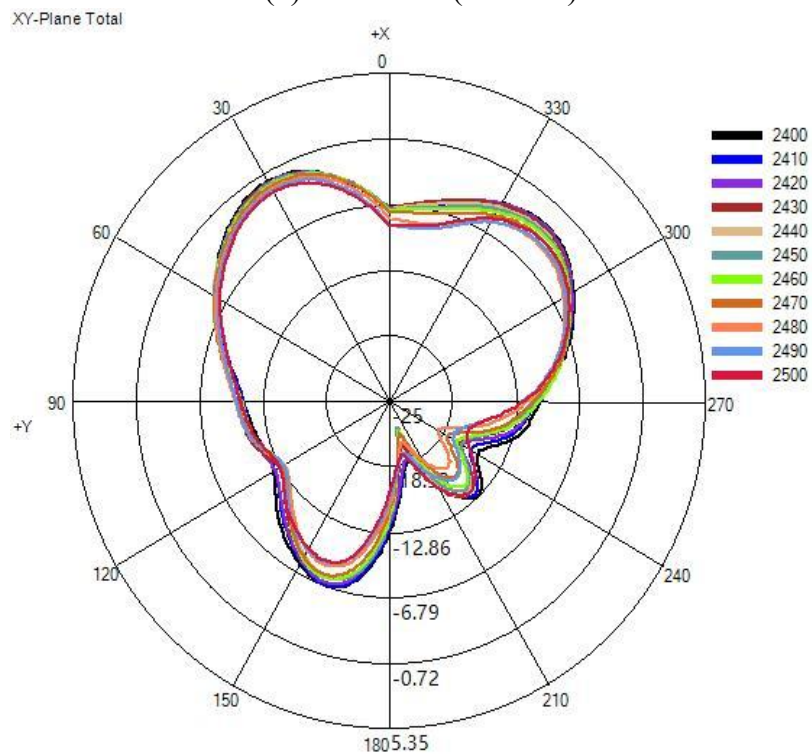
(7) X-Y Plane(unit:dBi):
