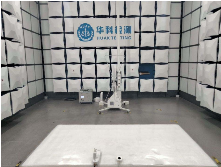
Model: X6 Pro Radiated Emissions
