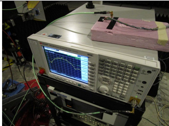
Conducted Setup
