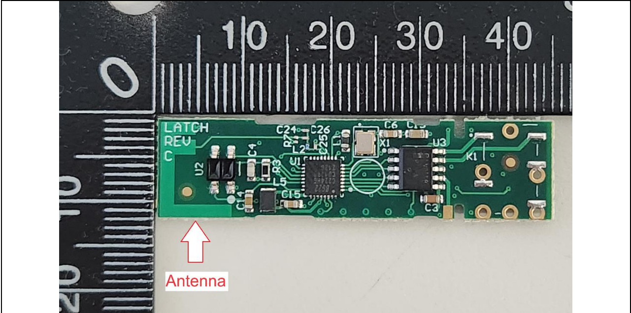
PCB Inverted F Antenna noted Top of EUT
