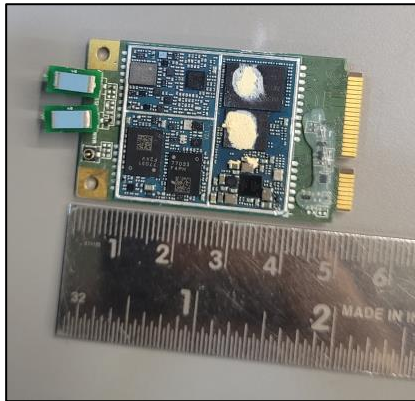
LTE Module front view with Dimesions
