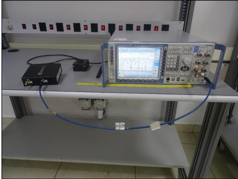
Cellular Conducted Test Setup
