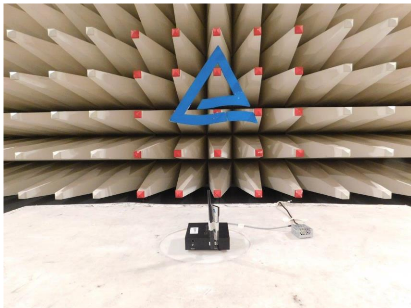
Radiated Test Setup
