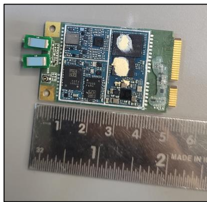
LTE Module front view with Dimensions
