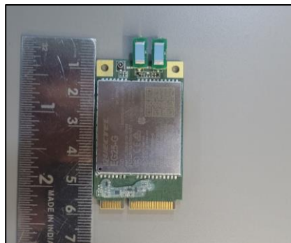
LTE Module Front View & Dimensions
