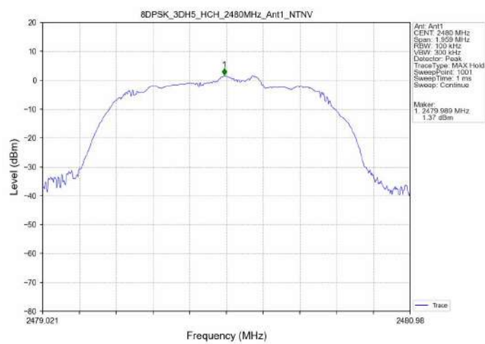
8DPSK_3DH5_HCH_2480MHz_Ant1_NTNV
