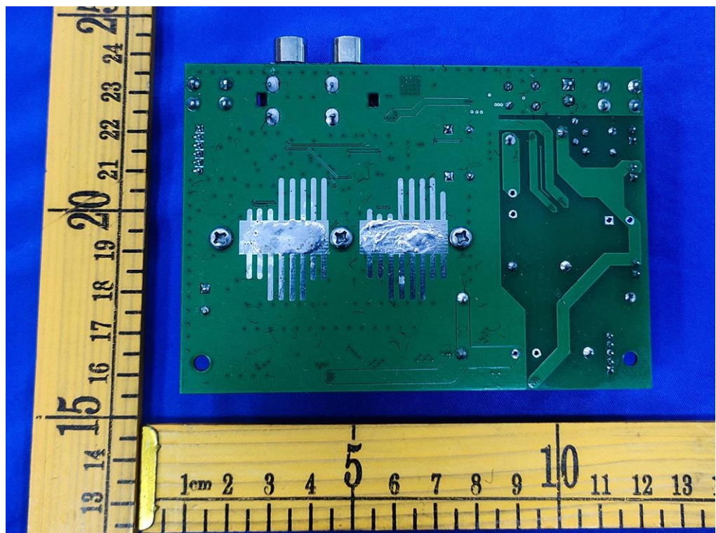
Model Classic B65A PCB view
