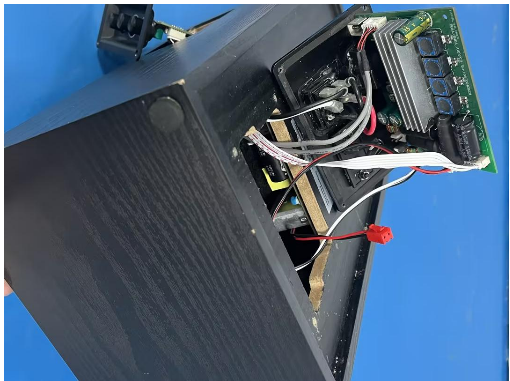
Model Classic B65A Interior view
