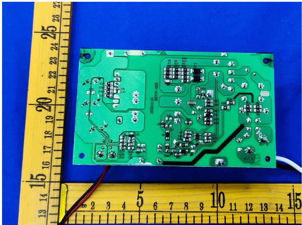
Model Classic B40A PCB view
