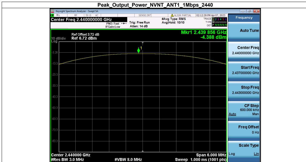
Peak_Output_Power_NVNT_ANT1_1Mbps_2440
