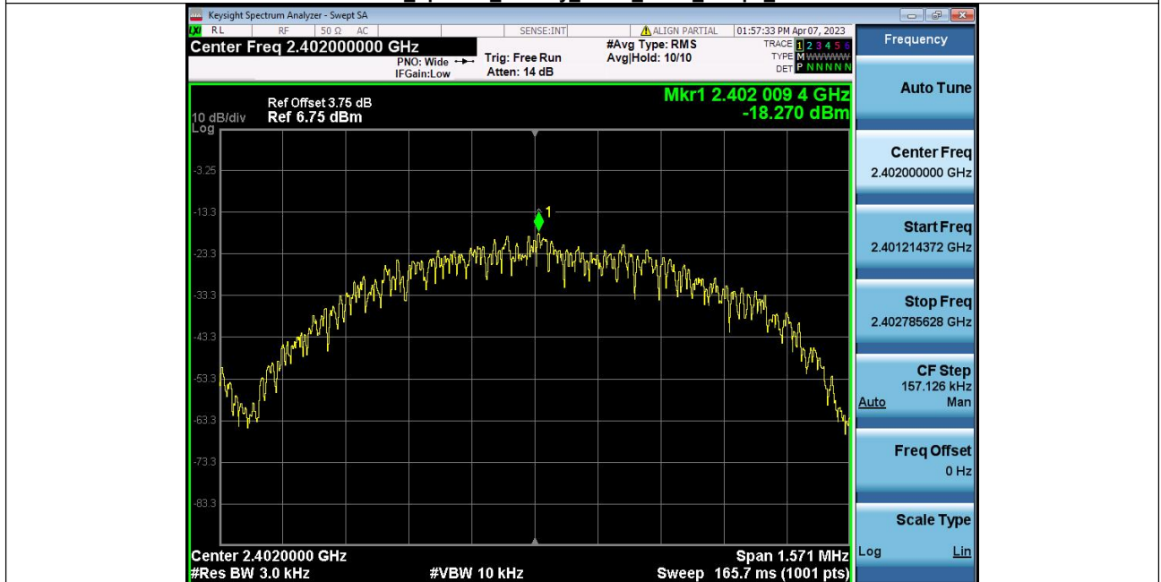
Power_Spectral_Density_NVNT_ANT1_1Mbps_2402
