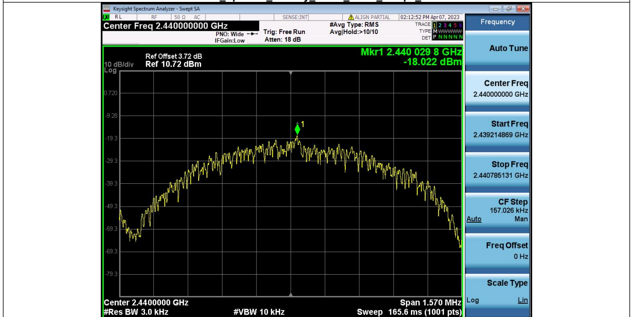
Power_Spectral_Density_NVNT_ANT1_1Mbps_2440
