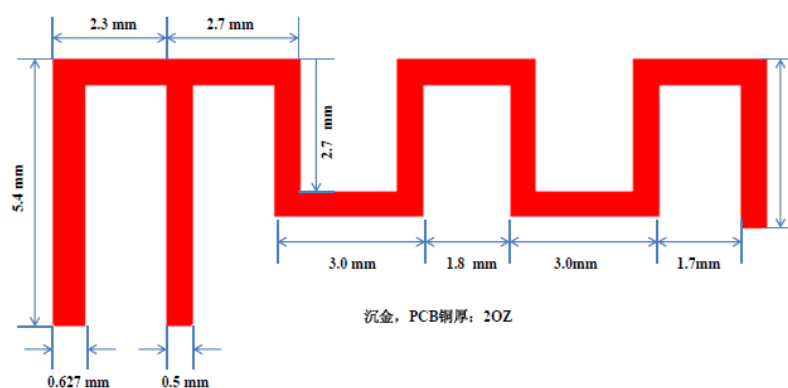
Picture 2 Antenna Dimension
