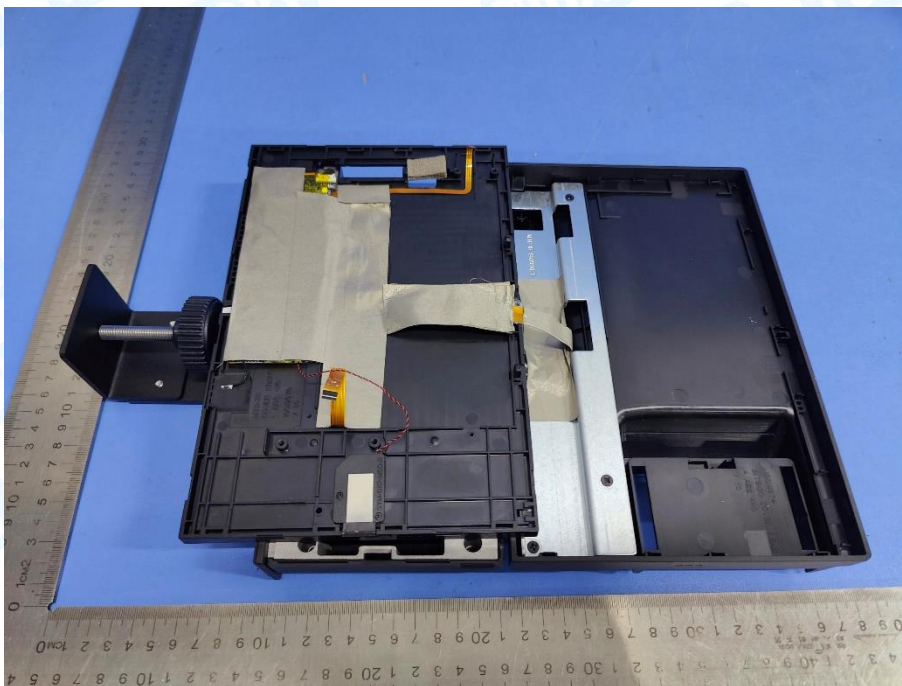
Photo 11 Internal of EUT (With Internal Battery)
