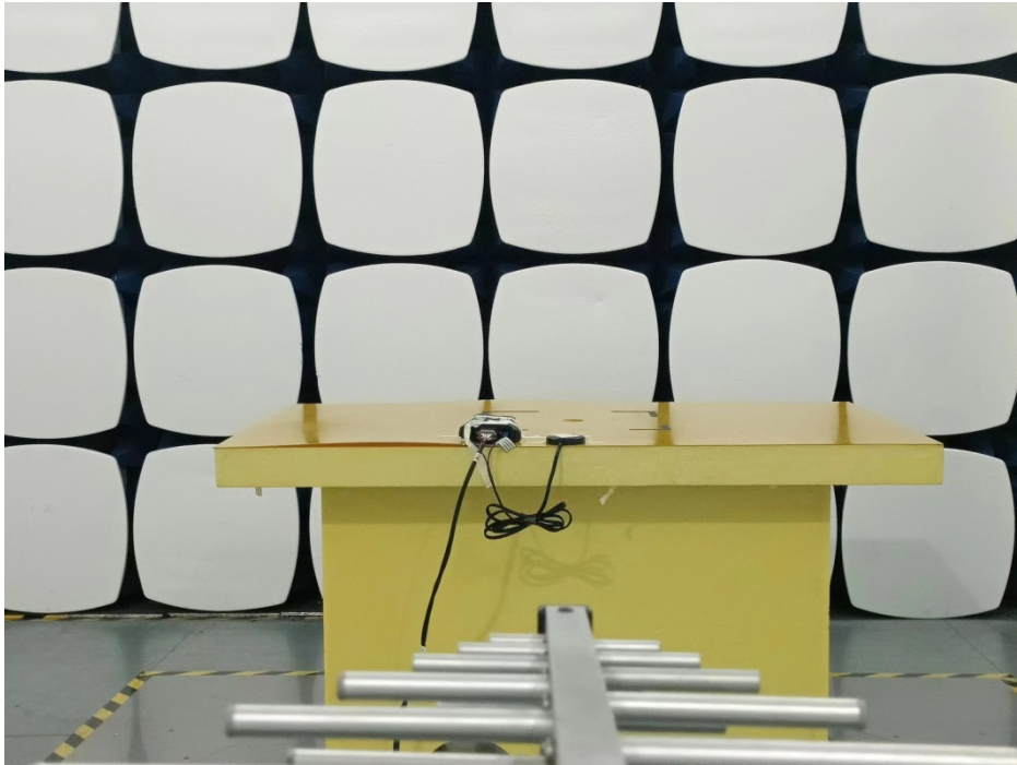
Below 1GHz
