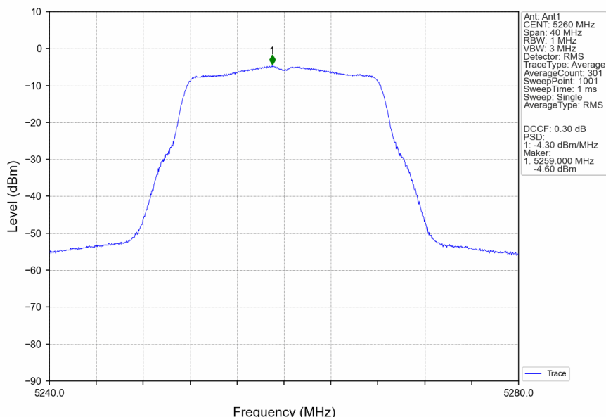
802.11a_LCH_5260MHz_Ant1_NTNV
