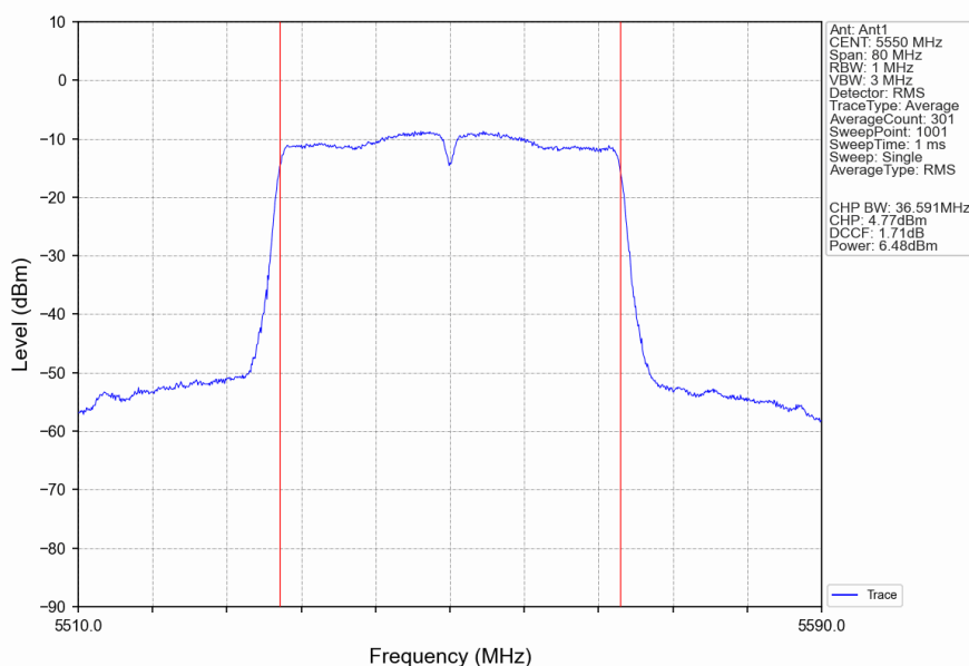
802.11n(HT40)_MCH_5550MHz_Ant1_NTNV
