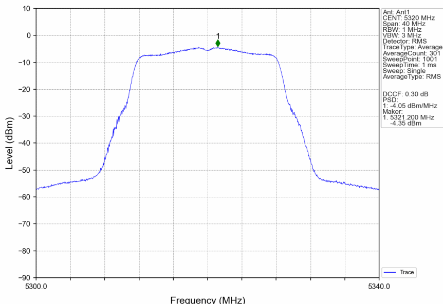
802.11a_HCH_5320MHz_Ant1_NTNV
