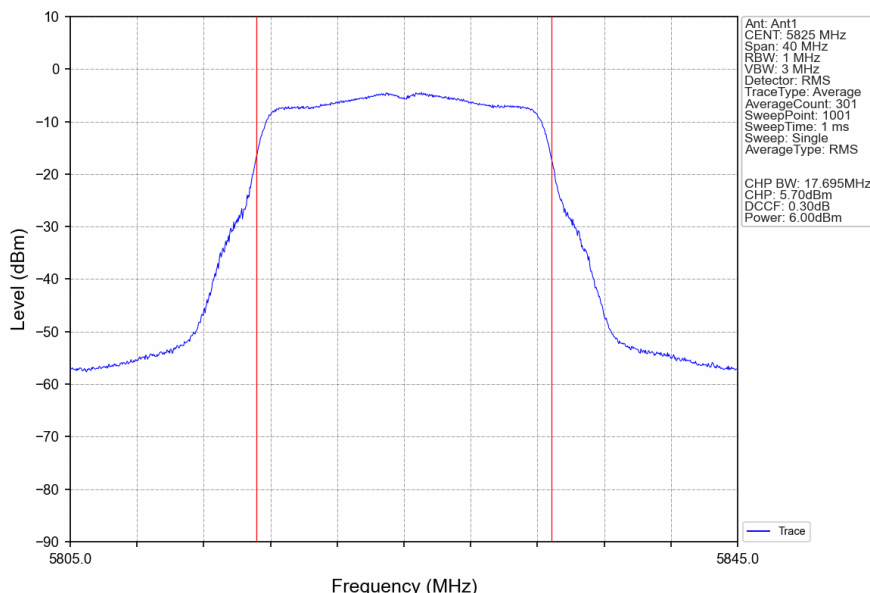
802.11a_HCH_5825MHz_Ant1_NTNV
