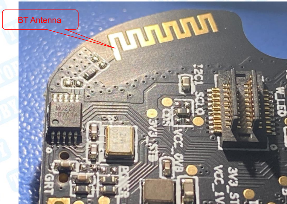
Photo 21 Appearance of PCB
