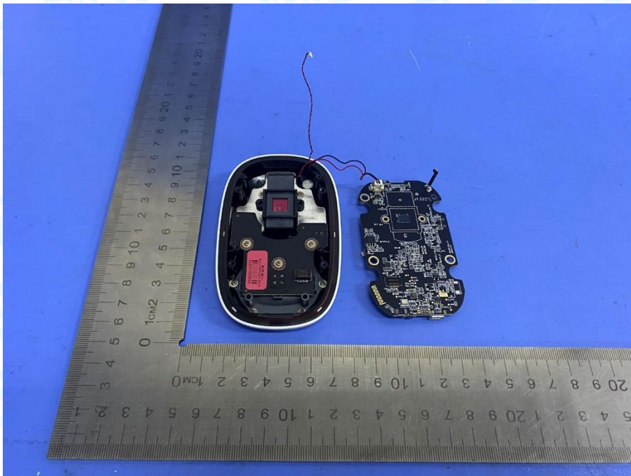
Photo 15 Internal of EUT
