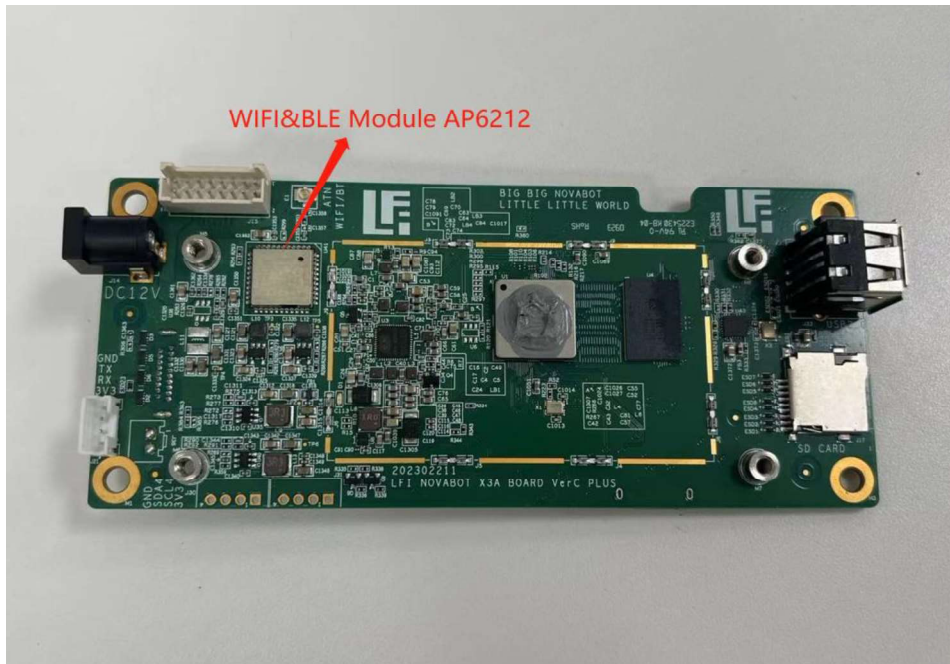
Internal: Top of X3A board
