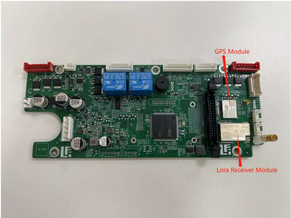
Internal: Top of Motor board
