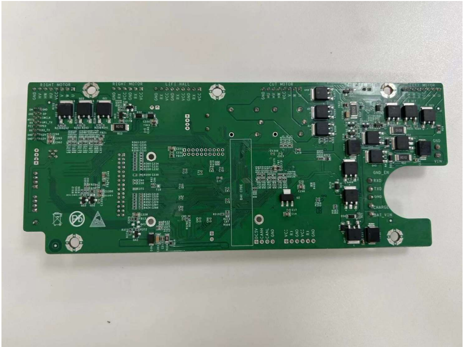
Internal: Bottom of Motor board
