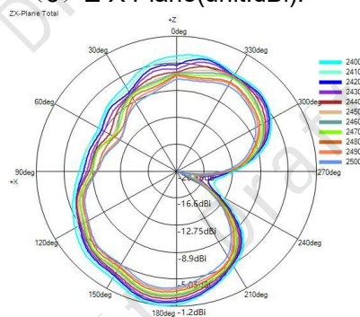
(3) Z-X Plane(unit:dBi):
