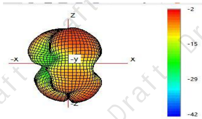
(5) Typical Free Space 3D Radiation Pattern at 2450MHz(unit:dBi)
