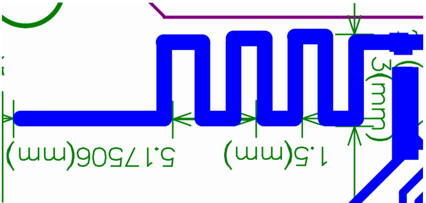
Figure Normal Module antenna
