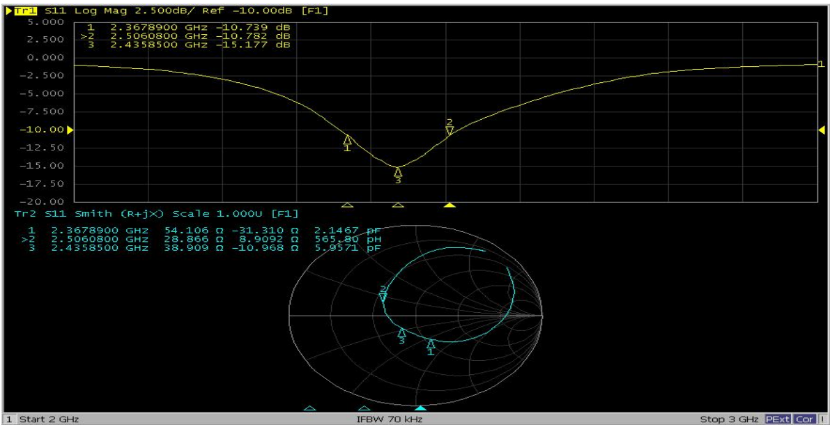
Figure Normal Module antenna S11
