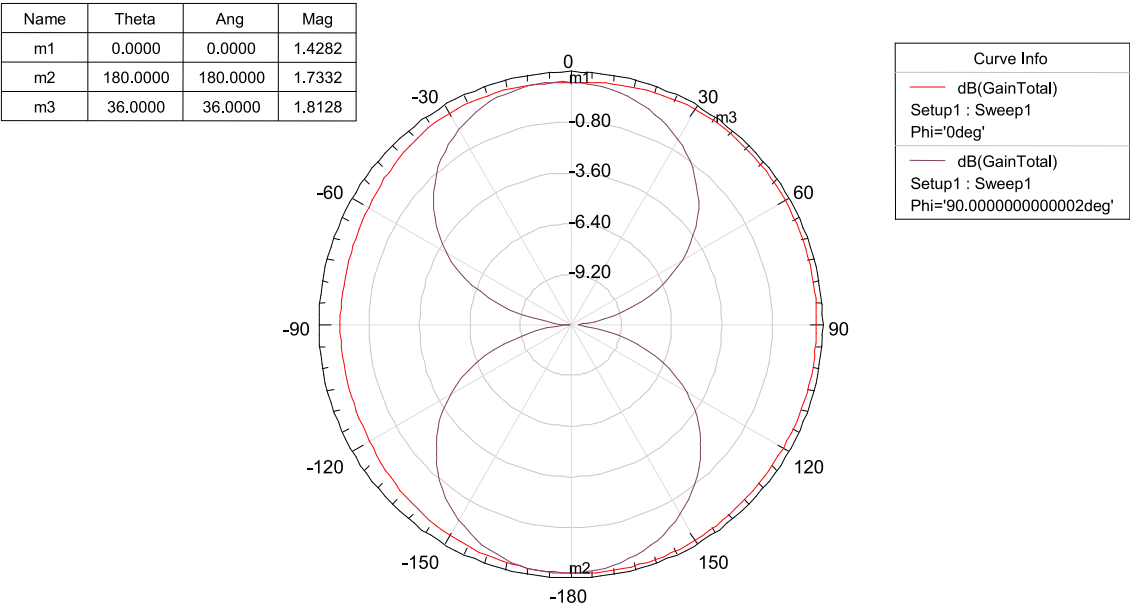
Radiation Patterns(GAIN @ 2440MHz)
