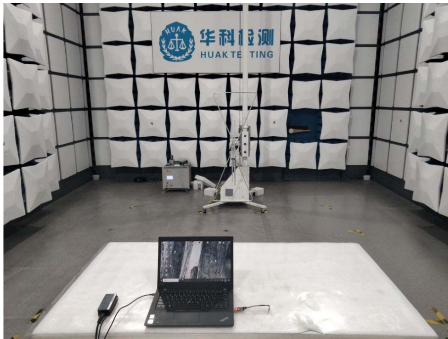
YTX51822-S02 Radiated Emissions
