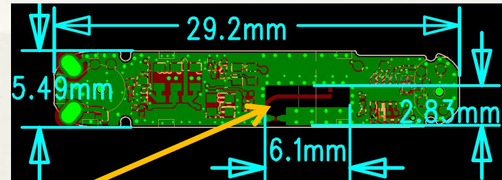
Right ear PCB
