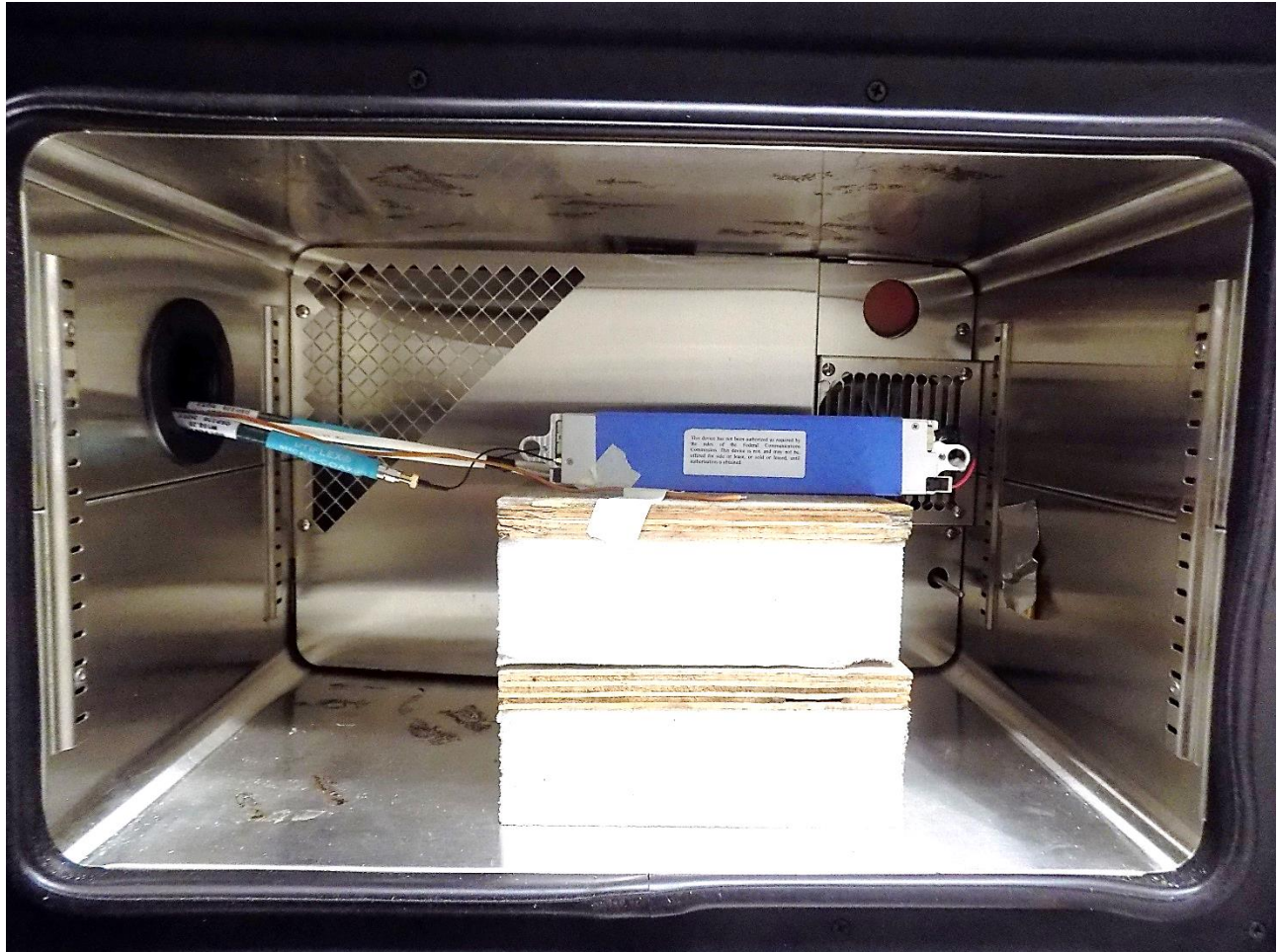
Figure 6: Test Setup for RF Conducted View
