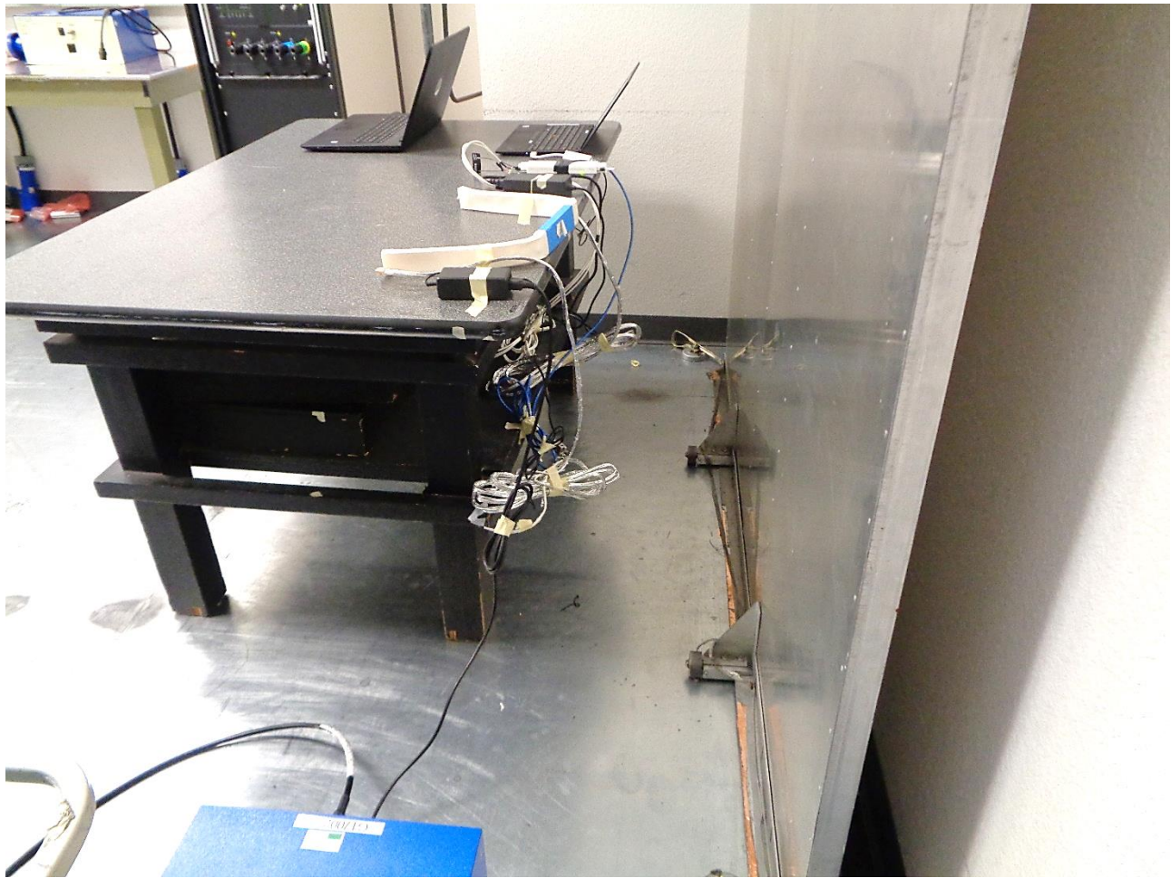
Figure 5: Test Setup for AC Conducted Emissions View 2
