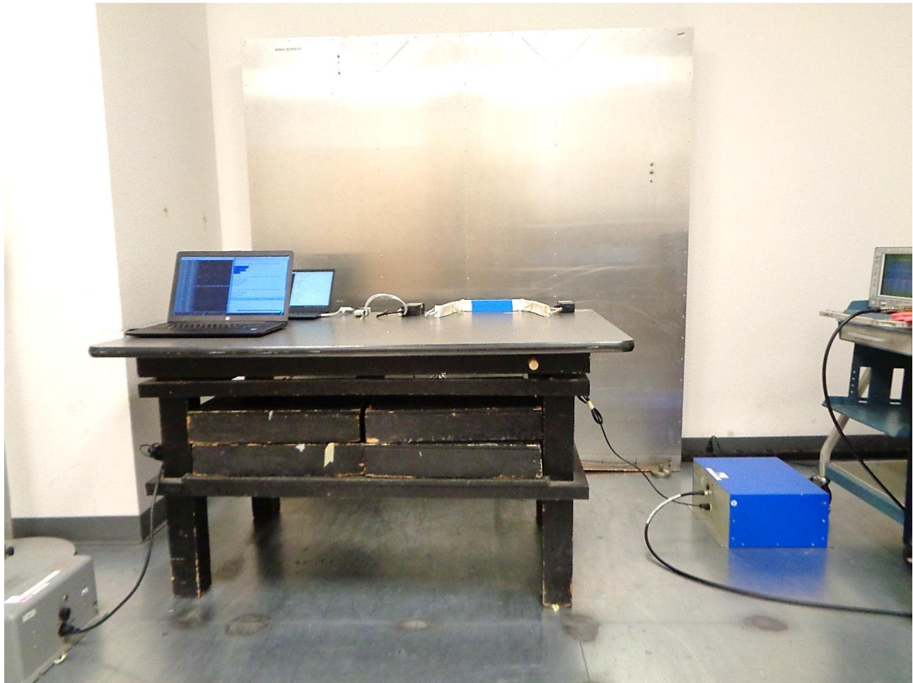
Figure 4: Test Setup for AC Conducted Emissions View 1
