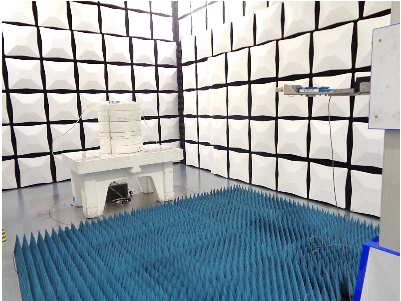
Figure 3: Test Setup for Radiated Emissions 18GHz to 40 GHz
