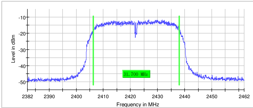
6 dB Bandwidth
