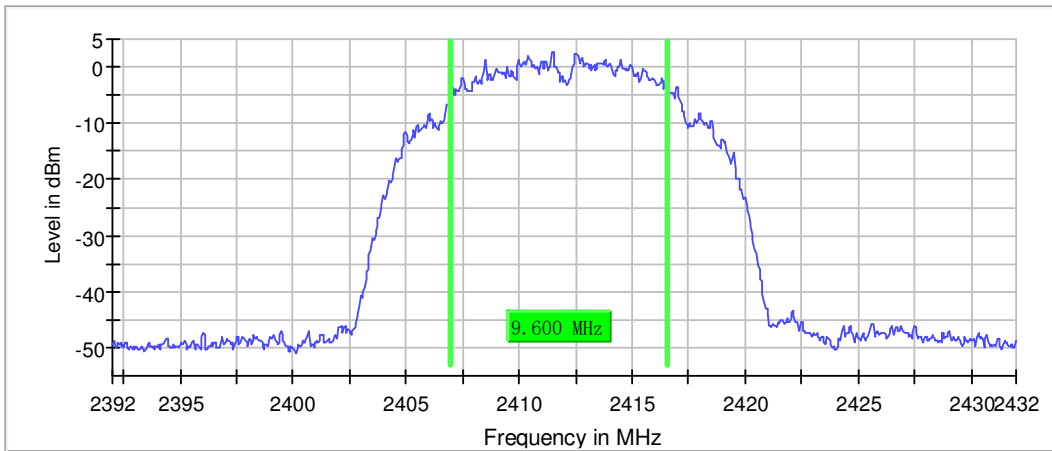
6 dB Bandwidth
