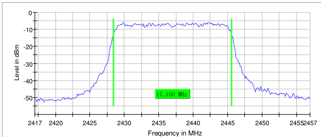
99 % Bandwidth
