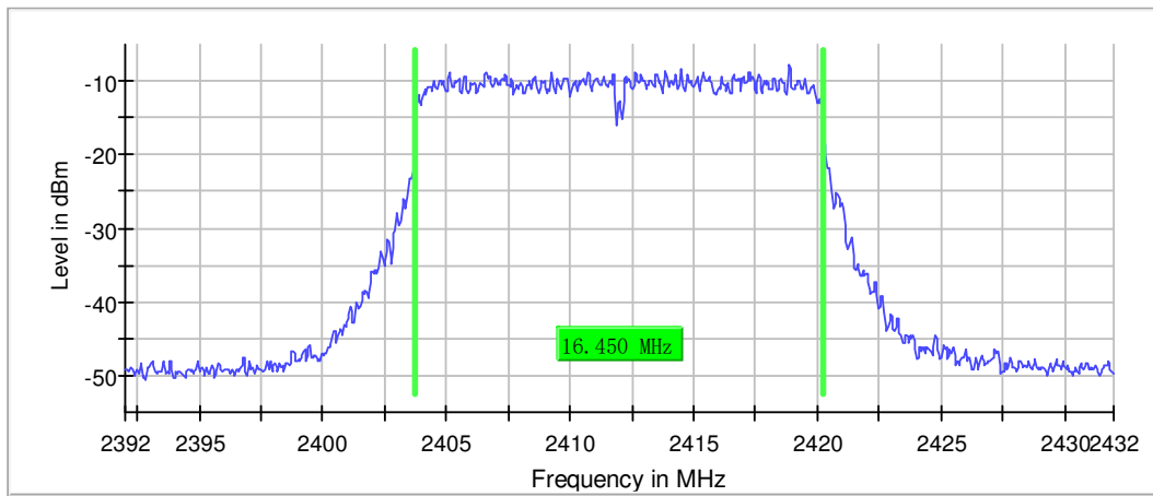
6 dB Bandwidth
