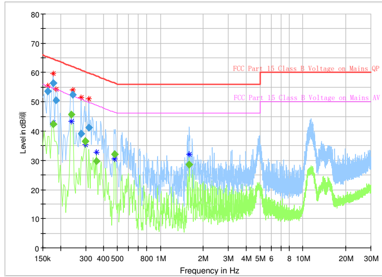
Full Spectrum
