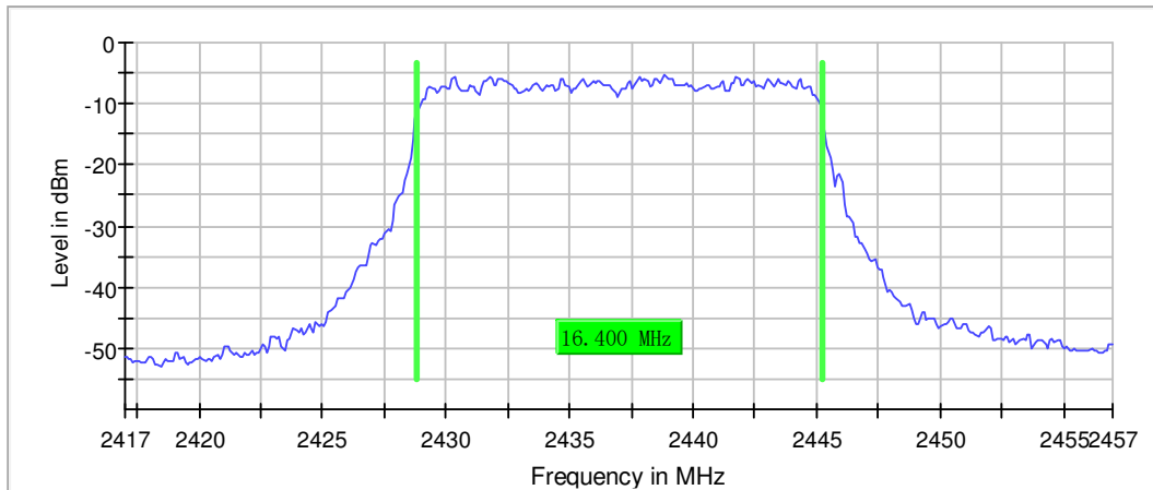
99 % Bandwidth
