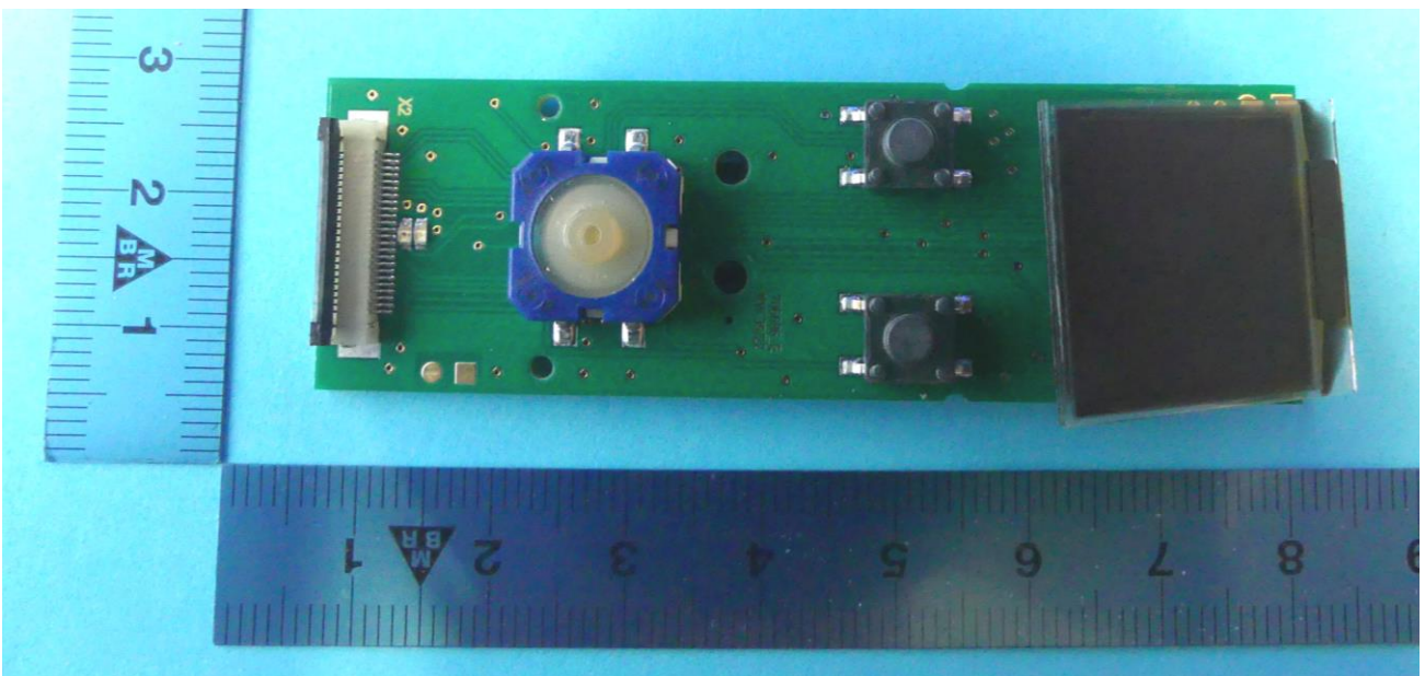
PCB Display top view
