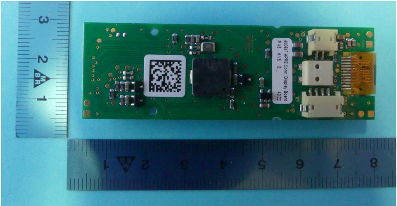
PCB Display bottom view
