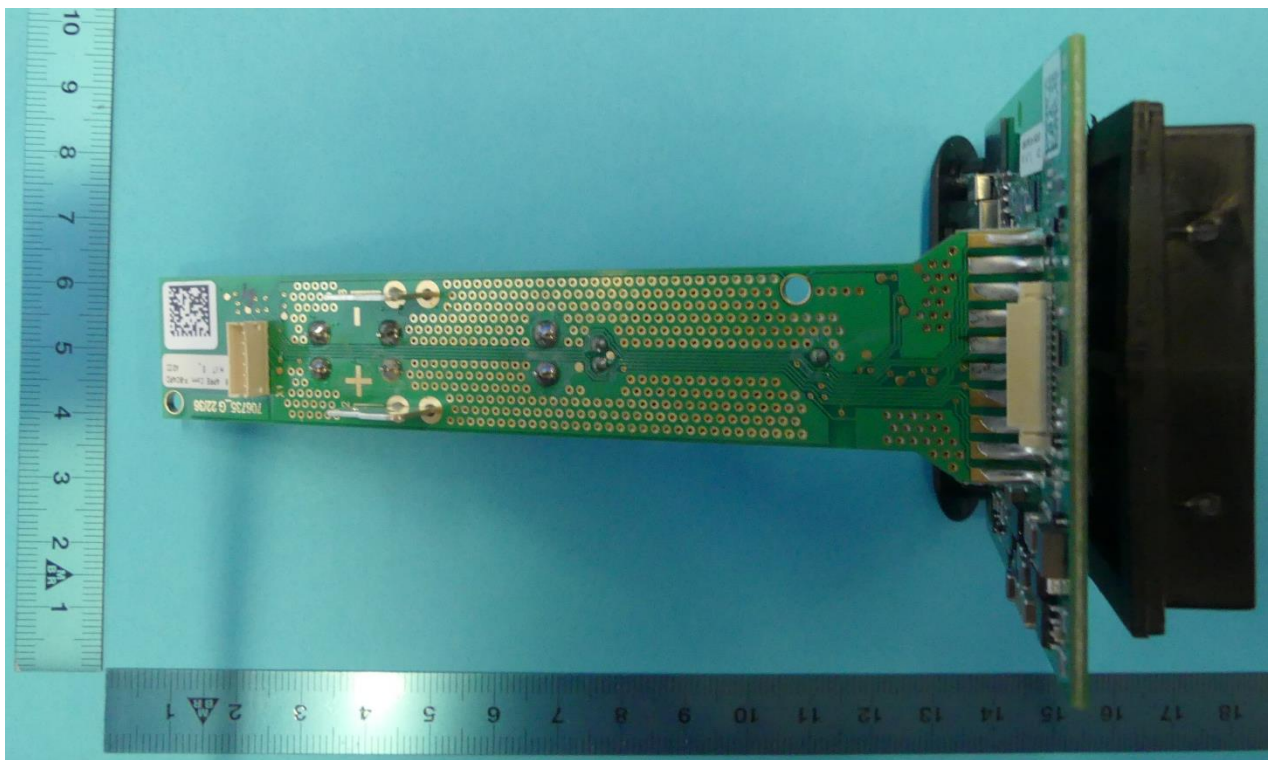
PBoard bottom view
