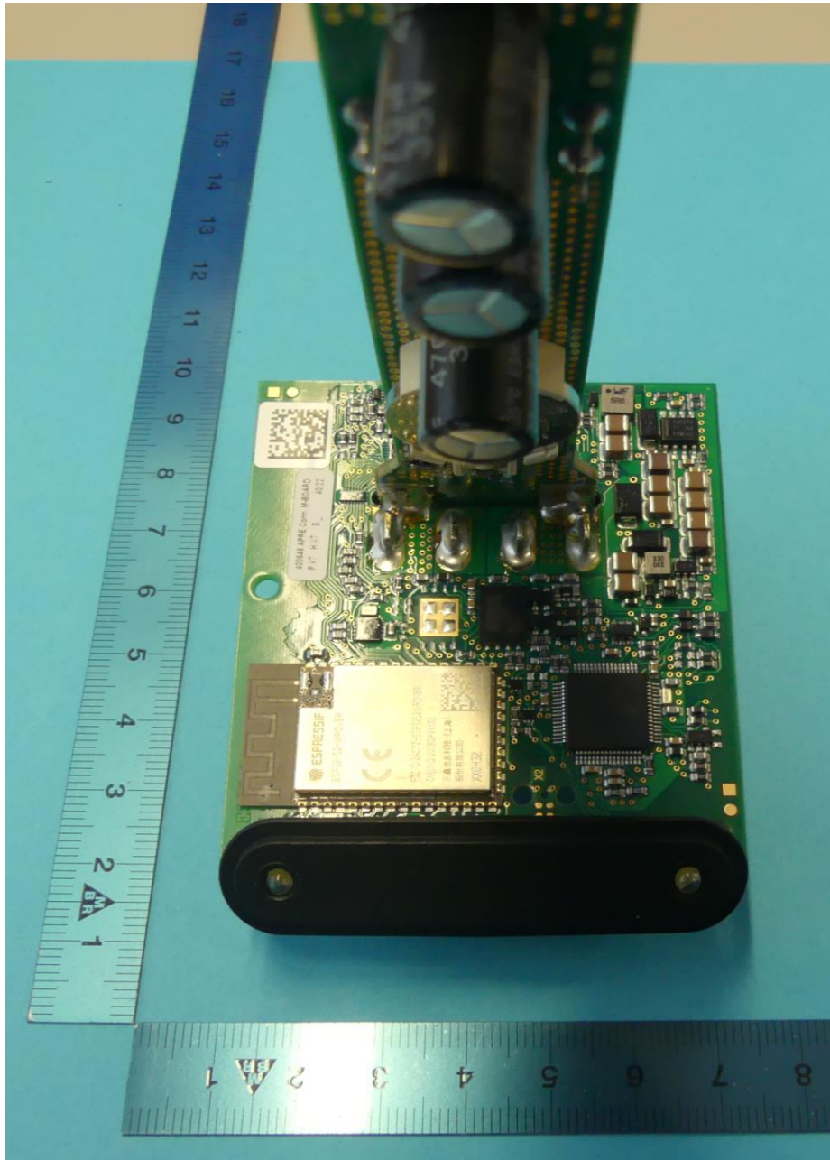
MBoard top view
