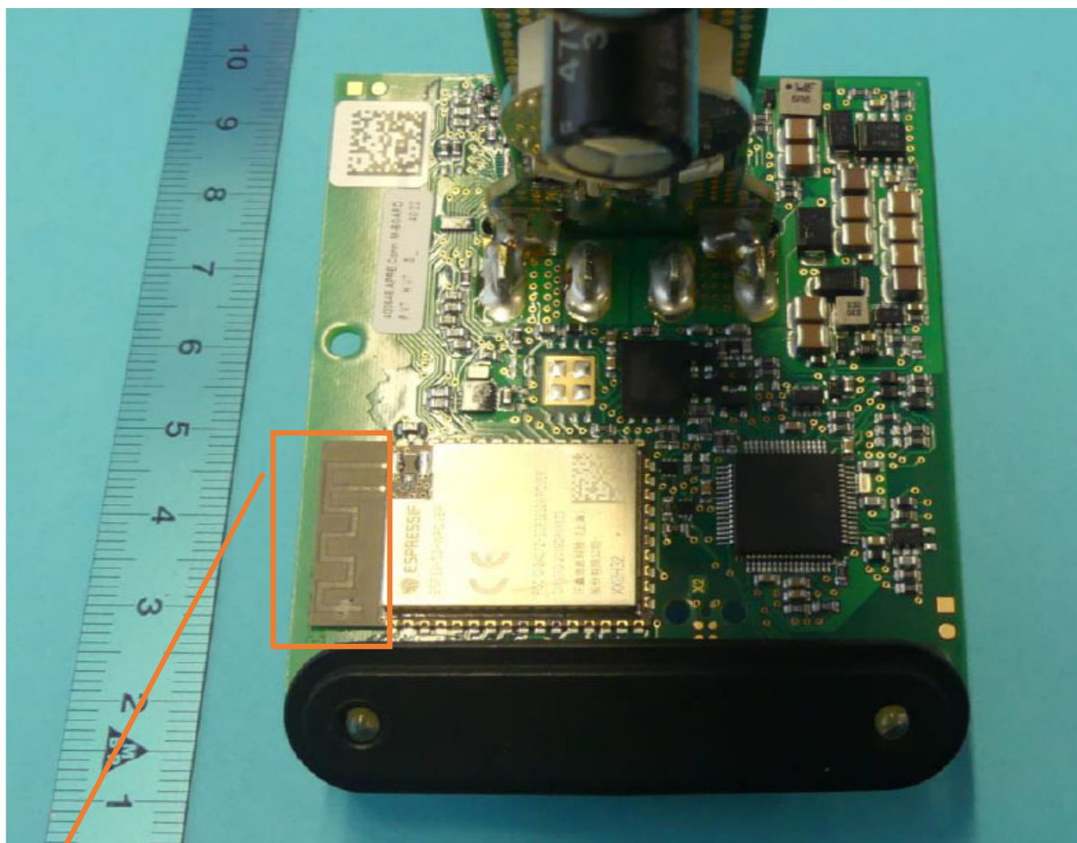
Antenna Position
