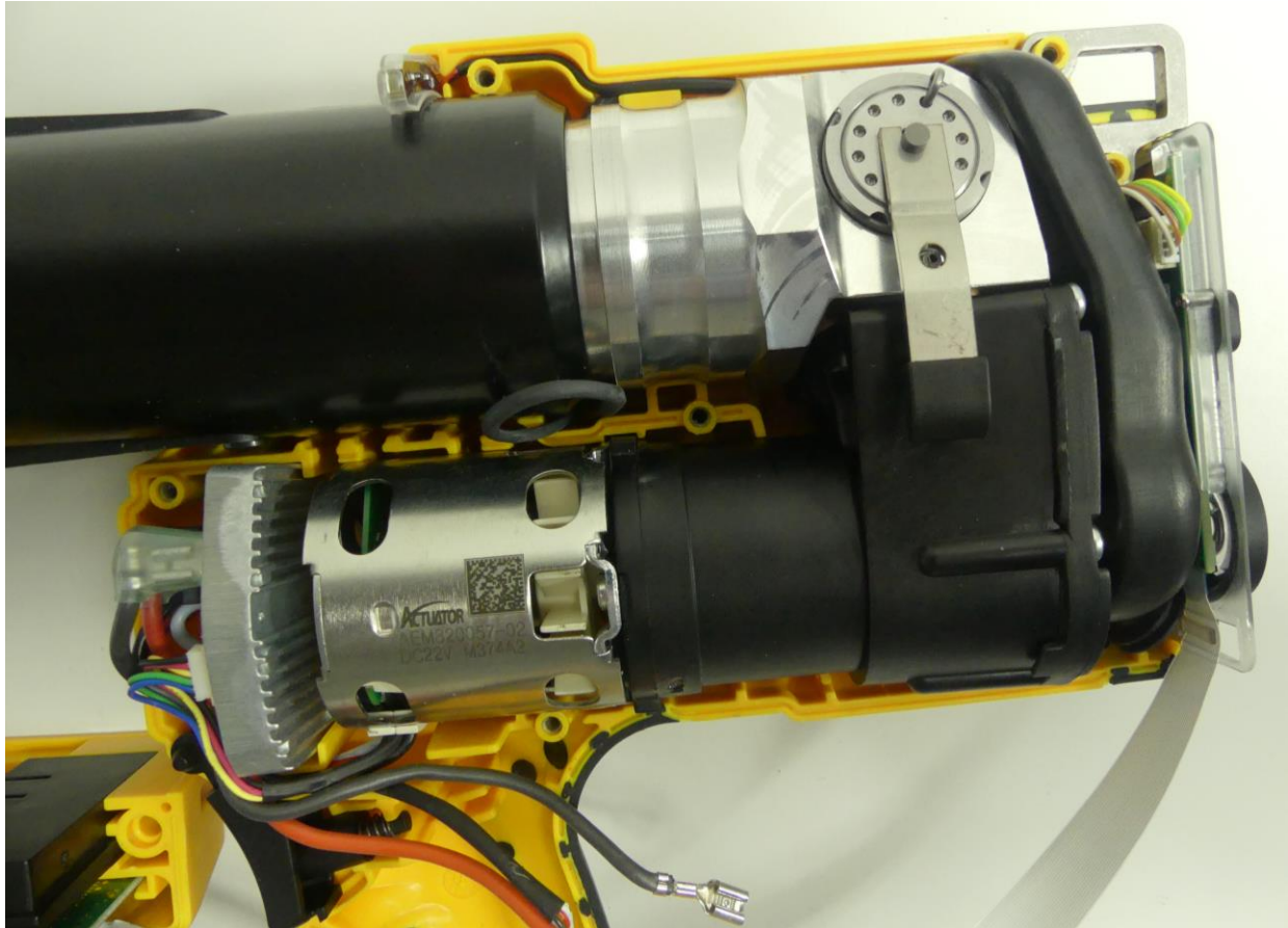
Hydraulic block, D.C. Motor
