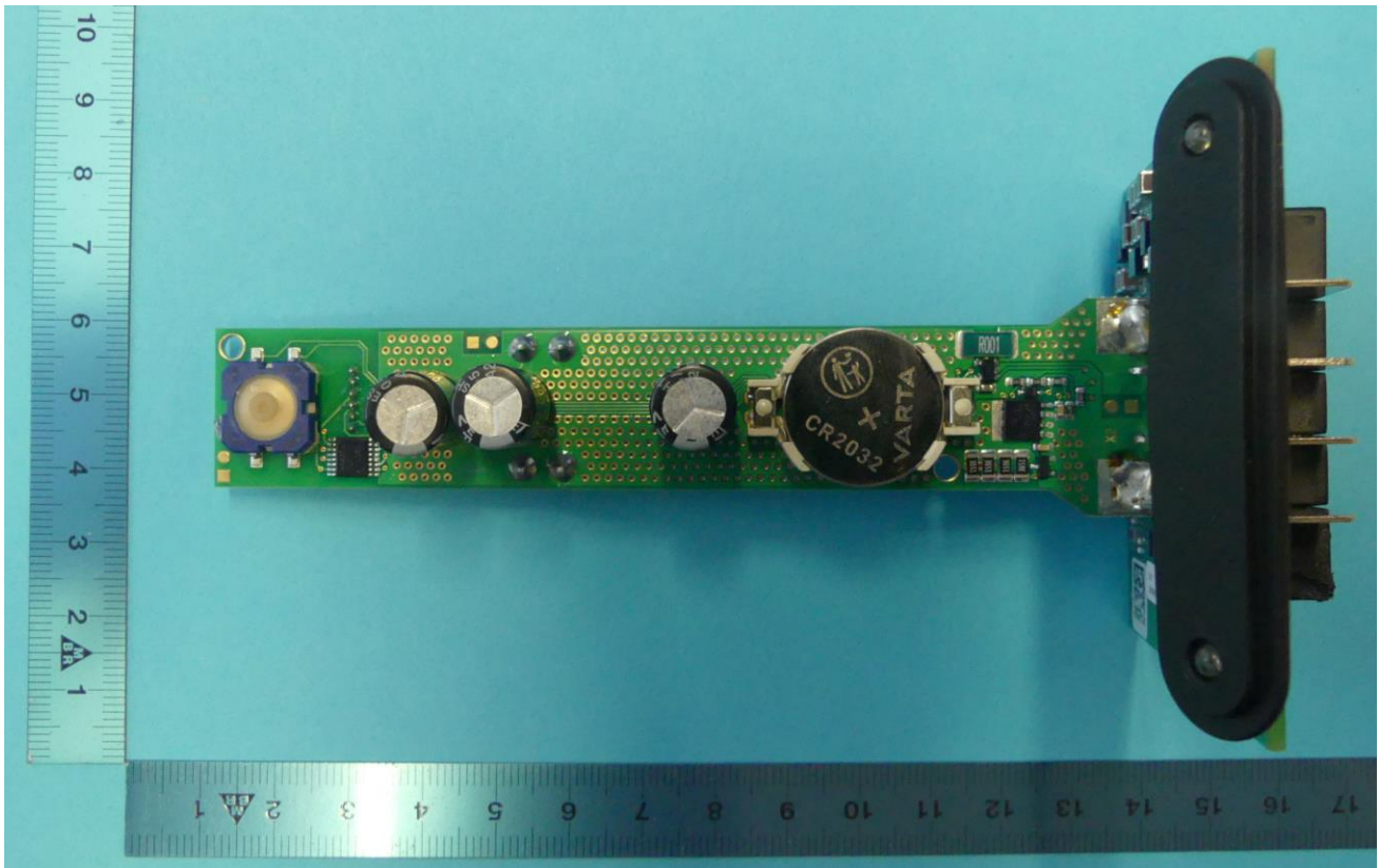
PBoard top view
