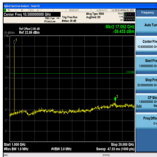
Band4-10MHz-16QAM-20175-50RB#0-Range2:1000~20000MHz
