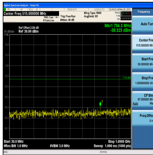
Band2-15MHz-16QAM-18900-75RB#0-Range1:30~1000MHz
