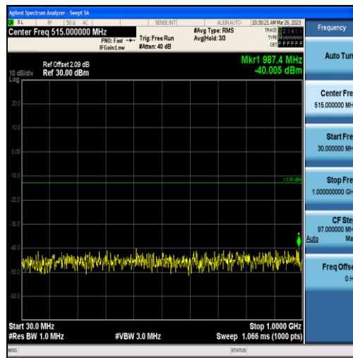
Band2-10MHz-QPSK-19150-50RB#0-Range1:30~1000MHz
