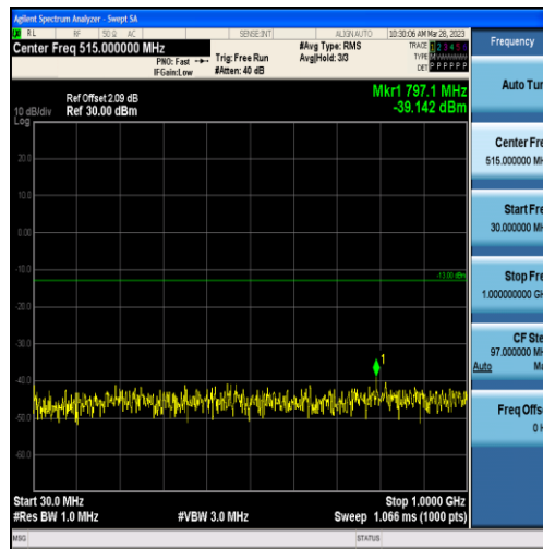
Band2-10MHz-16QAM-18900-50RB#0-Range1:30~1000MHz
