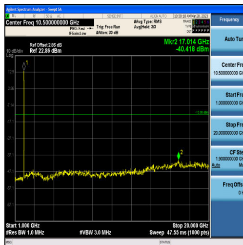
Band2-10MHz-16QAM-18900-50RB#0-Range2:1000~20000MHz
