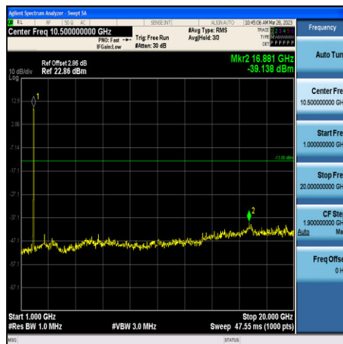
Band2-15MHz-16QAM-18900-75RB#0-Range2:1000~20000MHz
