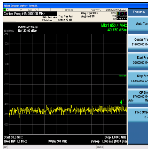
Band2-20MHz-16QAM-19100-100RB#0-Range1:30~1000MHz
