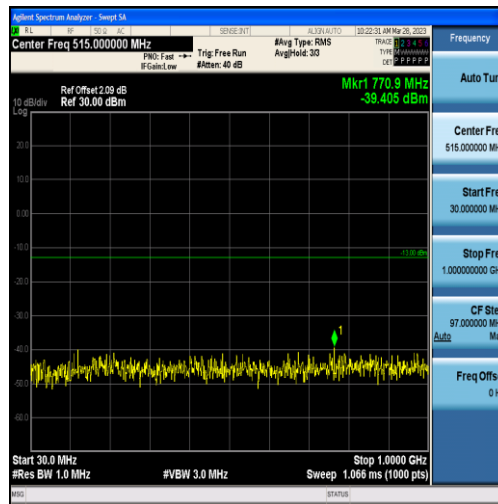
Band2-5MHz-16QAM-18900-25RB#0-Range1:30~1000MHz
