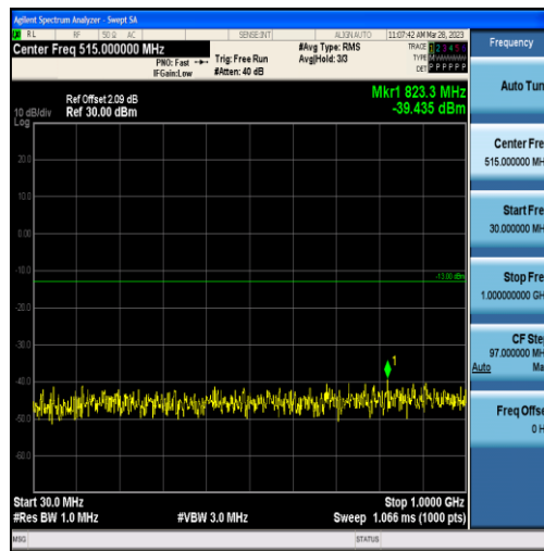
Band4-1.4MHz-16QAM-19957-6RB#0-Range1:30~1000MHz
