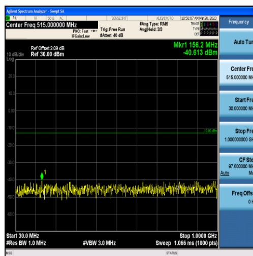
Band2-20MHz-QPSK-18900-100RB#0-Range1:30~1000MHz
