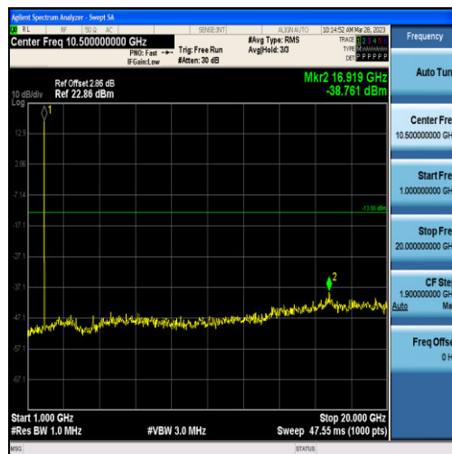
Band2-3MHz-16QAM-18900-15RB#0-Range2:1000~20000MHz
