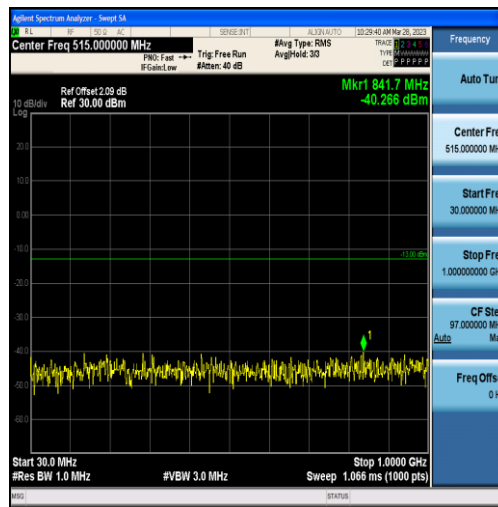
Band2-10MHz-16QAM-18650-50RB#0-Range1:30~1000MHz
