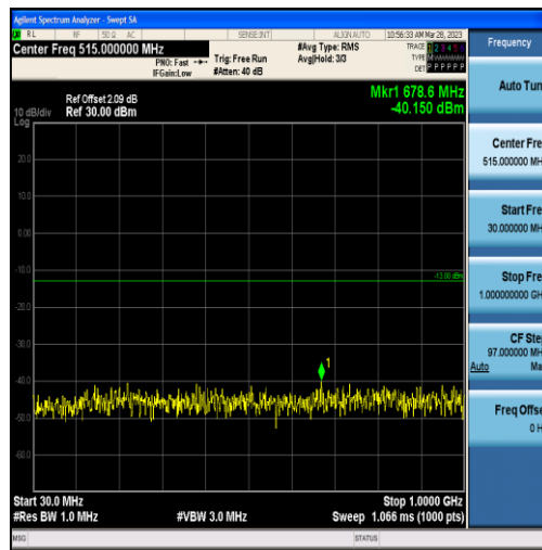
Band2-20MHz-QPSK-19100-100RB#0-Range1:30~1000MHz
