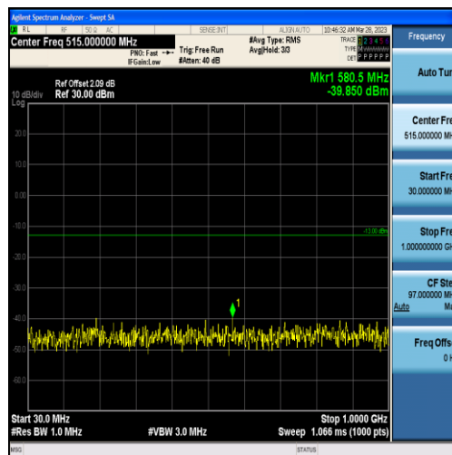
Band2-15MHz-16QAM-19125-75RB#0-Range1:30~1000MHz
