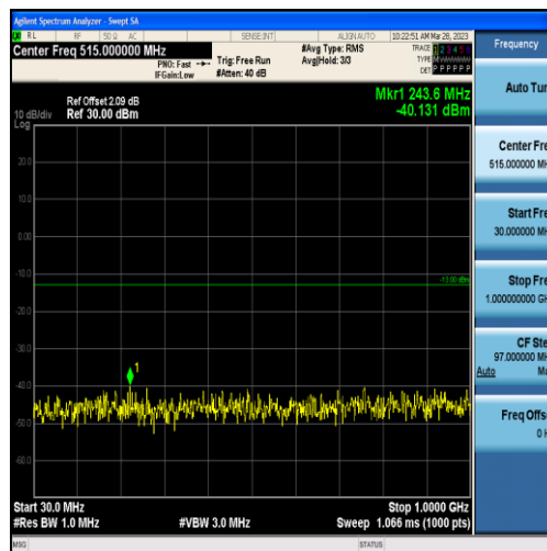
Band2-5MHz-16QAM-19175-25RB#0-Range1:30~1000MHz
