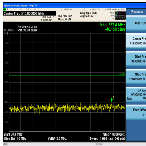
Band4-1.4MHz-QPSK-20175-6RB#0-Range1:30~1000MHz
