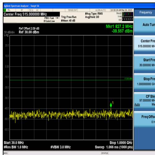
Band2-10MHz-16QAM-19150-50RB#0-Range1:30~1000MHz
