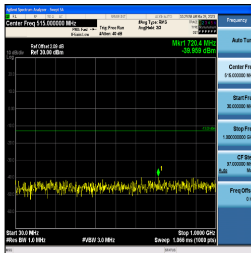
Band2-10MHz-QPSK-18900-50RB#0-Range1:30~1000MHz
