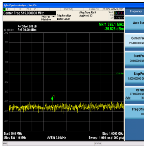
Band2-20MHz-16QAM-18700-100RB#0-Range1:30~1000MHz
