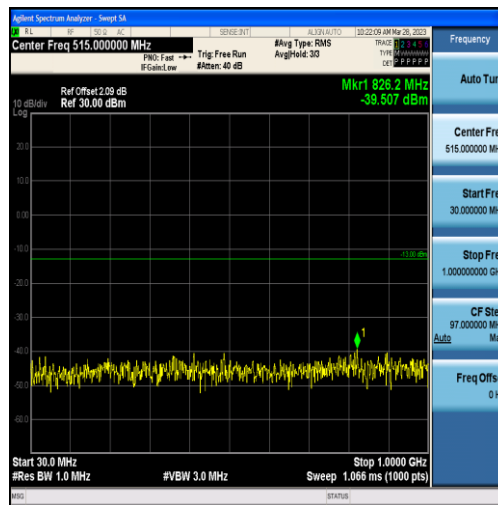
Band2-5MHz-16QAM-18625-25RB#0-Range1:30~1000MHz
