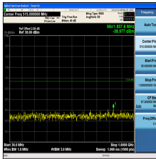
Band2-5MHz-QPSK-19175-25RB#0-Range1:30~1000MHz
