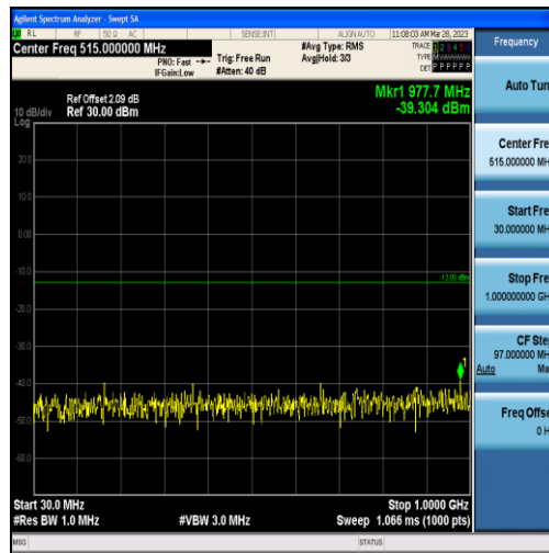
Band4-1.4MHz-16QAM-20175-6RB#0-Range1:30~1000MHz
