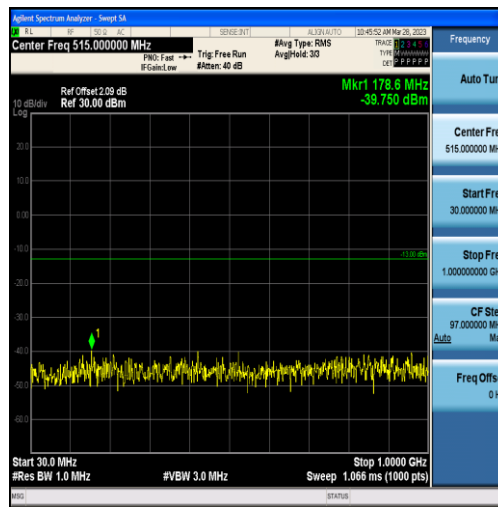
Band2-15MHz-QPSK-19125-75RB#0-Range1:30~1000MHz
