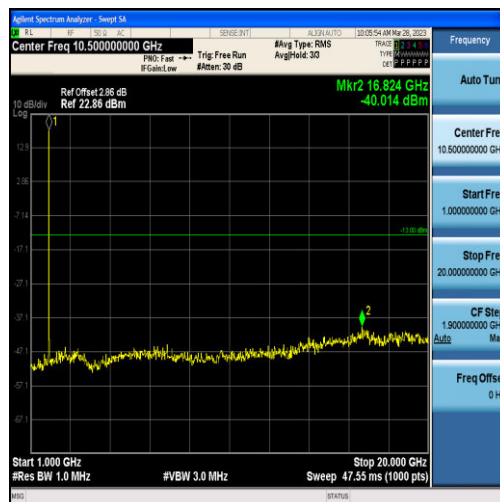
Band2-1.4MHz-16QAM-18900-6RB#0-Range2:1000~20000MHz
