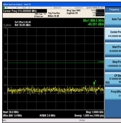
Band2-15MHz-16QAM-18675-75RB#0-Range1:30~1000MHz
