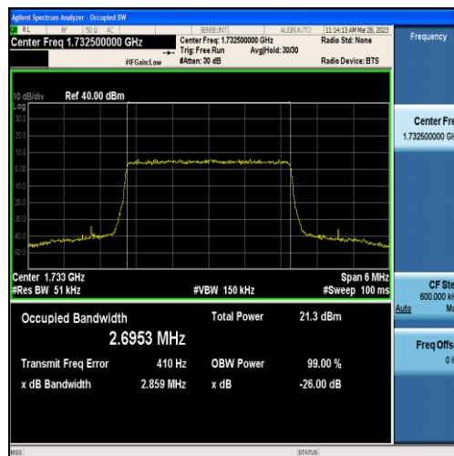
Band4-3MHz-QPSK-20175-15RB#0-2.6953
