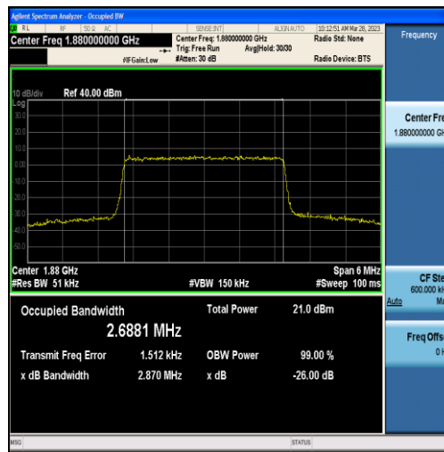
Band2-3MHz-16QAM-18900-15RB#0-2.6881
