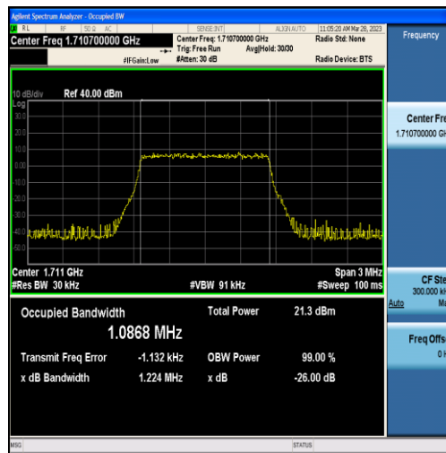
Band4-1.4MHz-QPSK-19957-6RB#0-1.0868
