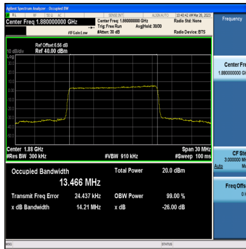
Band2-15MHz-16QAM-18900-75RB#0-13.466
