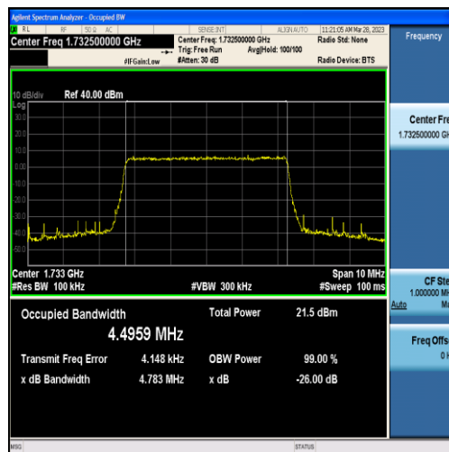
Band4-5MHz-QPSK-20175-25RB#0-4.4959
