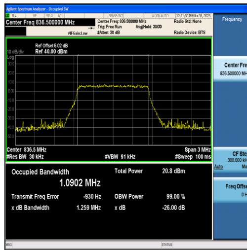
Band5-1.4MHz-16QAM-20525-6RB#0-1.0902
