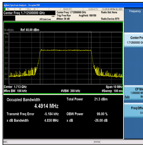
Band4-5MHz-QPSK-19975-25RB#0-4.4914
