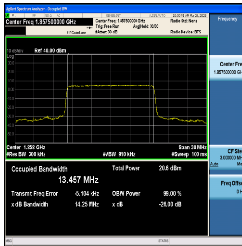
Band2-15MHz-QPSK-18675-75RB#0-13.457
