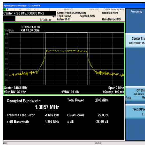
Band5-1.4MHz-16QAM-20643-6RB#0-1.0857
