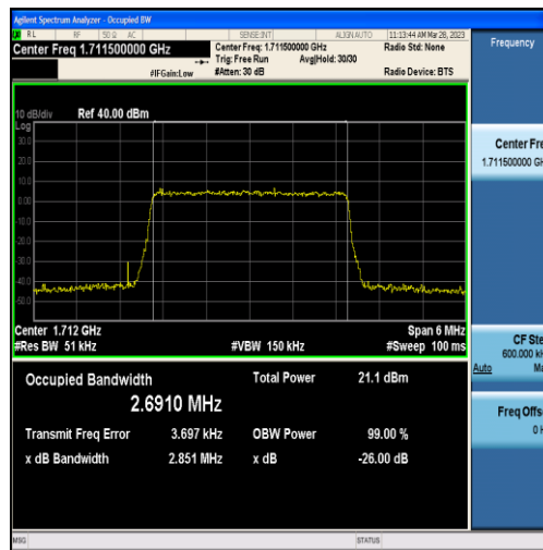
Band4-3MHz-QPSK-19965-15RB#0-2.6910
