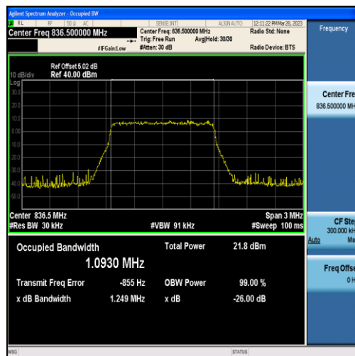
Band5-1.4MHz-QPSK-20525-6RB#0-1.0930
