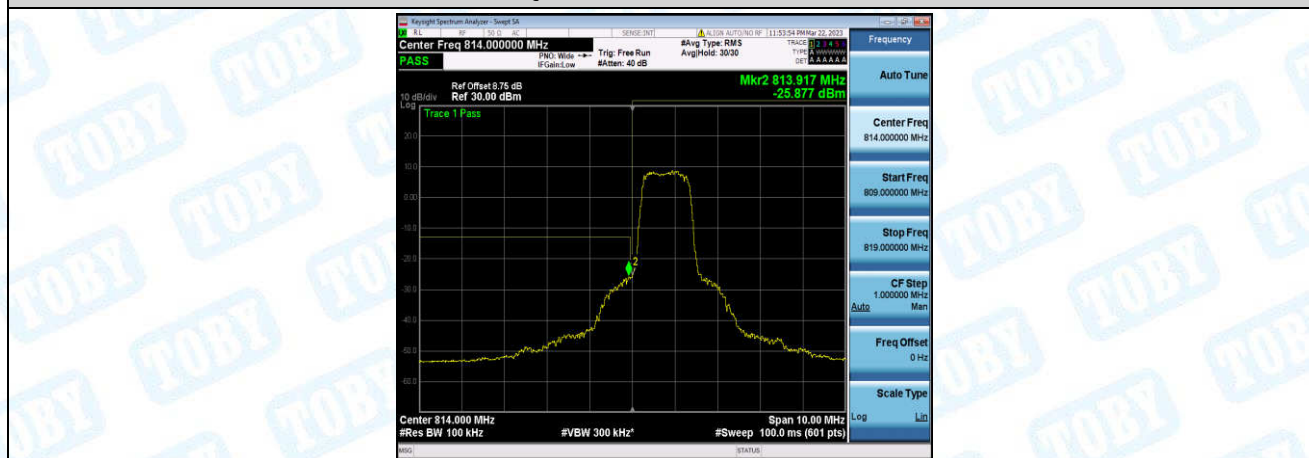
Band26-5MHz-16QAM-26715-6-0-Low--25.54,-25.88-PASS
