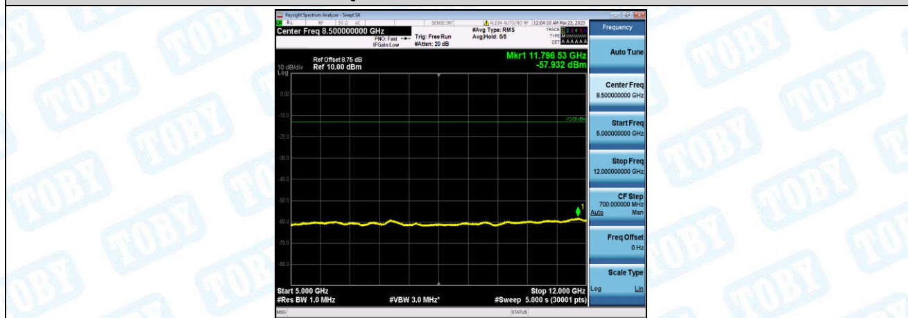
Band26-5MHz-16QAM-26715-1-0-Low-5000-12000--57.93-PASS
