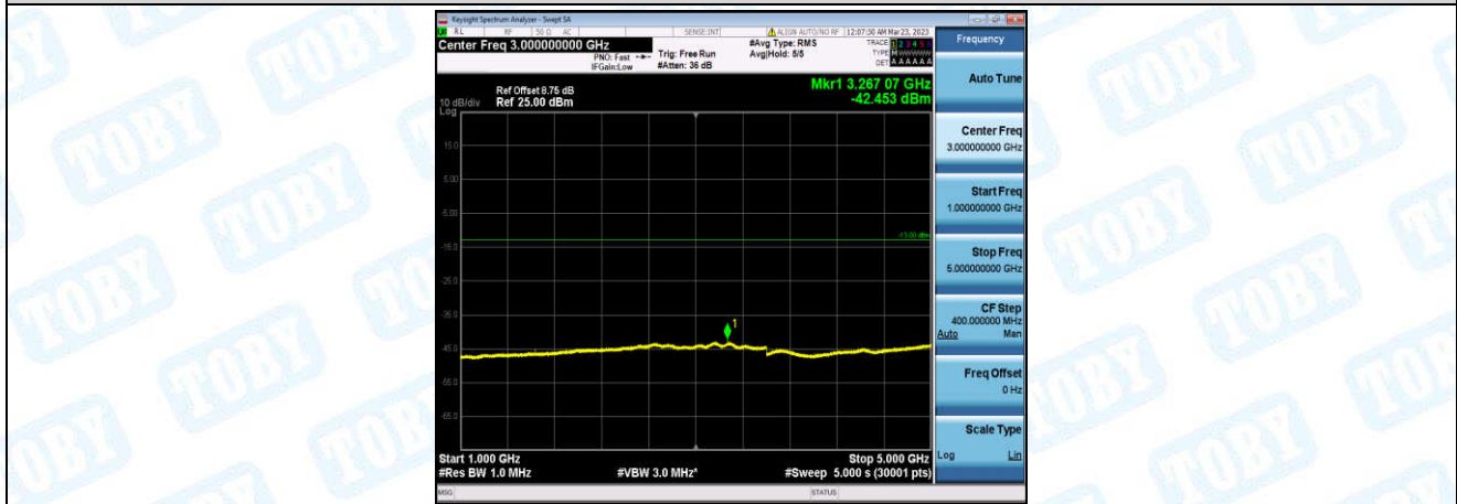
Band26-5MHz-16QAM-26740-1-0-Low-1000-5000--42.45-PASS
