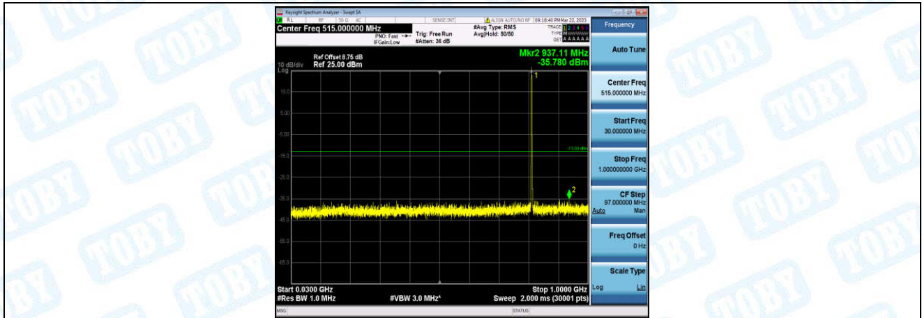
Band26-1.4MHz-16QAM-26697-1-0-Low-30-1000--35.78-PASS
