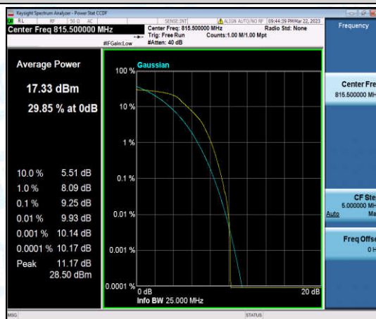
Band26-3MHz-QPSK-26705-6-0-Low-9.25-=<=13-PASS
