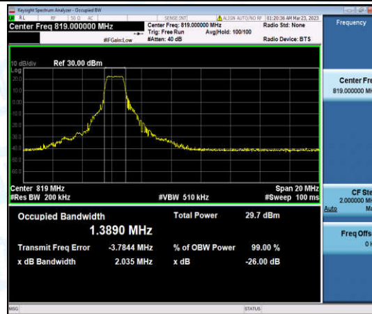
Band26-10MHz-16QAM-26740-6-0-Low-1.3890-2.035-PASS
