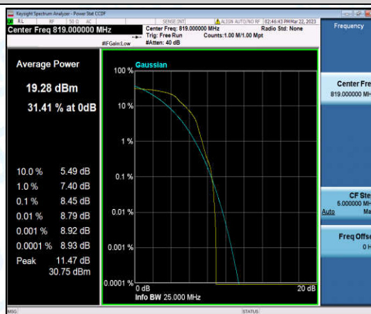
Band26-1.4MHz-QPSK-26740-1-0-Low-8.45-<=13-PASS
