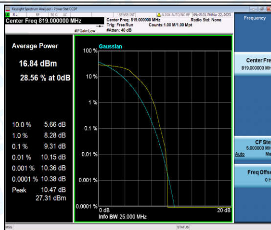
Band26-3MHz-16QAM-26740-6-0-Low-9.31-<=13-PASS
