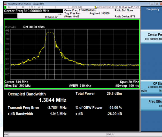
Band26-10MHz-QPSK-26740-6-0-Low-1.3844-1.913-PASS
